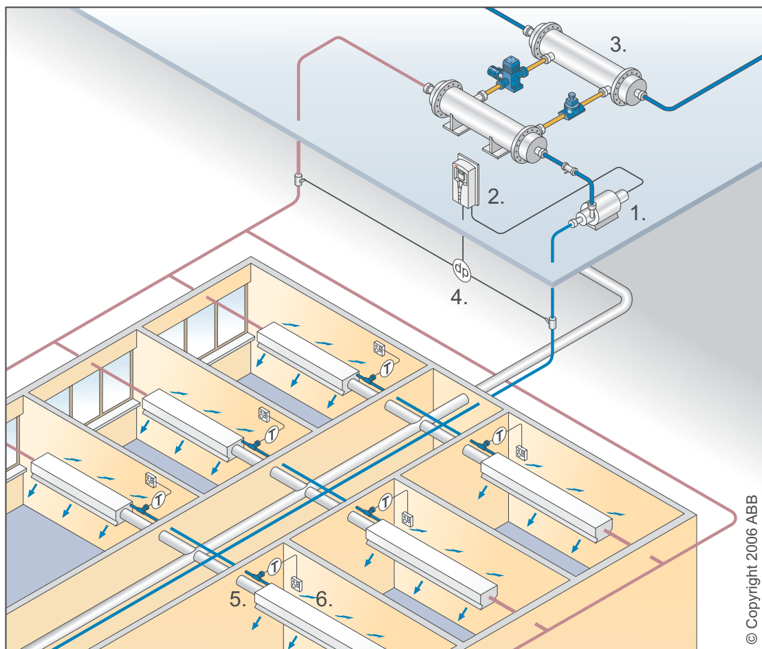
Chilled water system with variable speed drives.
