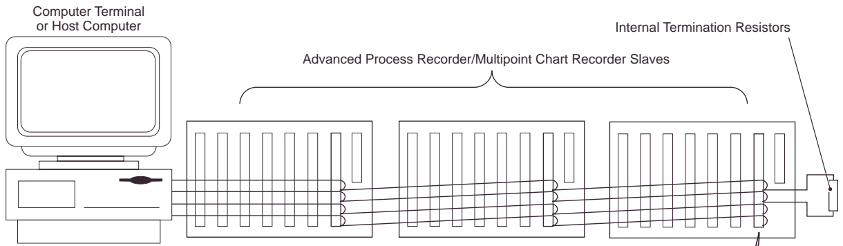
A – Schematic Diagram
