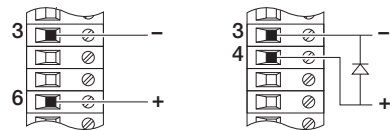
b – Voltage c – Current (non 2-wire Transmitters)
