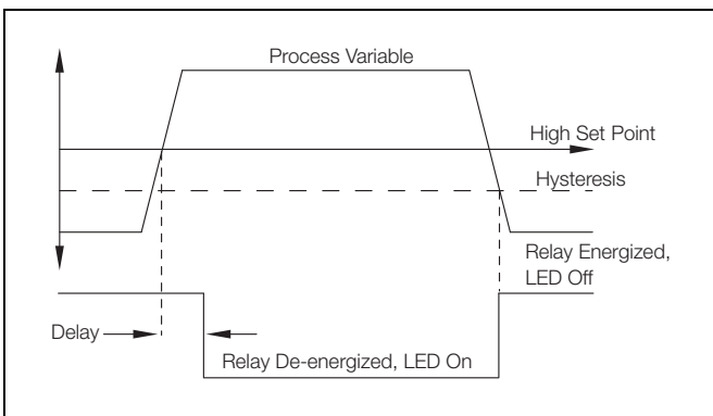
Fig. 5.3 High Failsafe Alarm with Hysteresis and Delay
