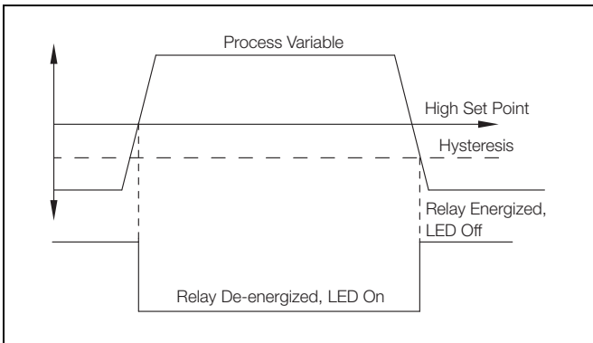
Fig. 5.2 High Failsafe Alarm with Hysteresis but no Delay
