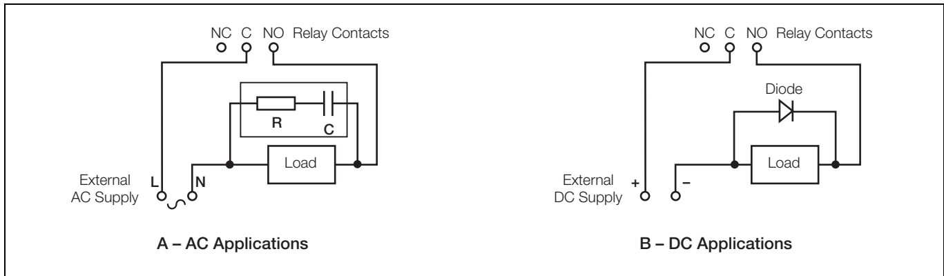
Fig. 6.6 Relay Contact Protection
