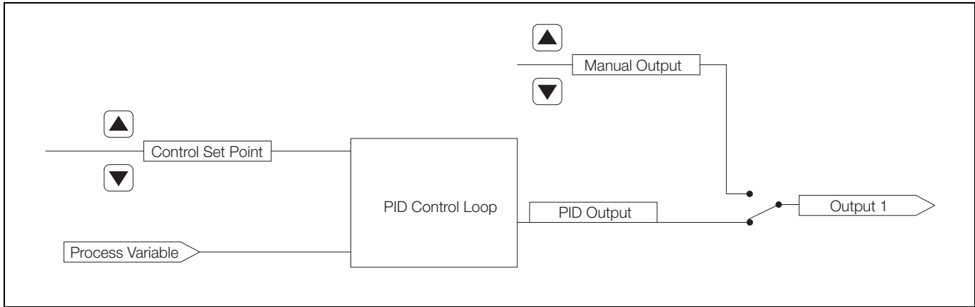
Fig. B.1 Single PID Controller
