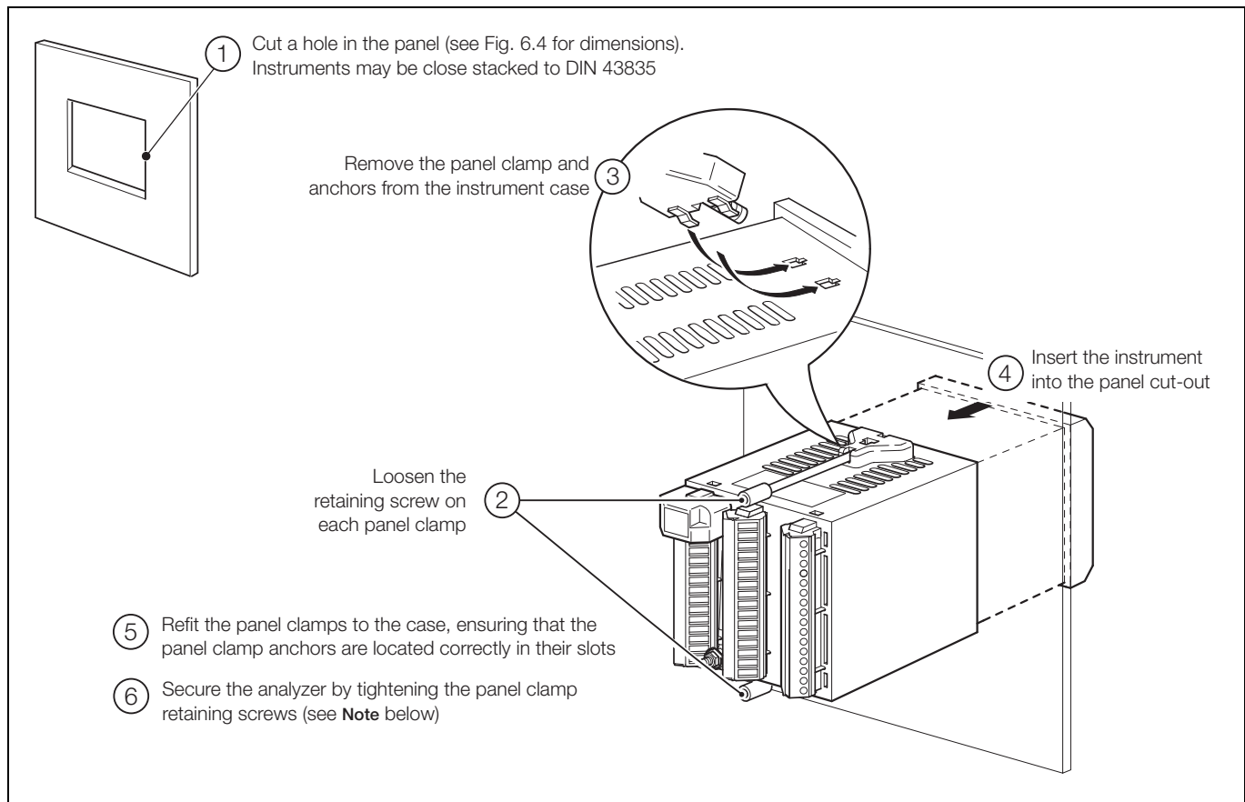
Fig. 6.5 Panel-mounting
