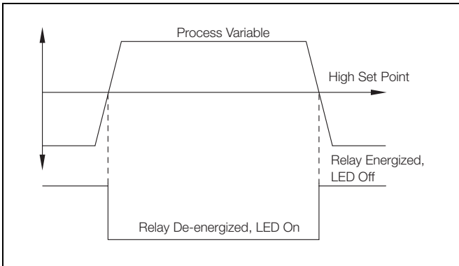
Fig. 5.1 High Failsafe Alarm without Hysteresis and Delay
