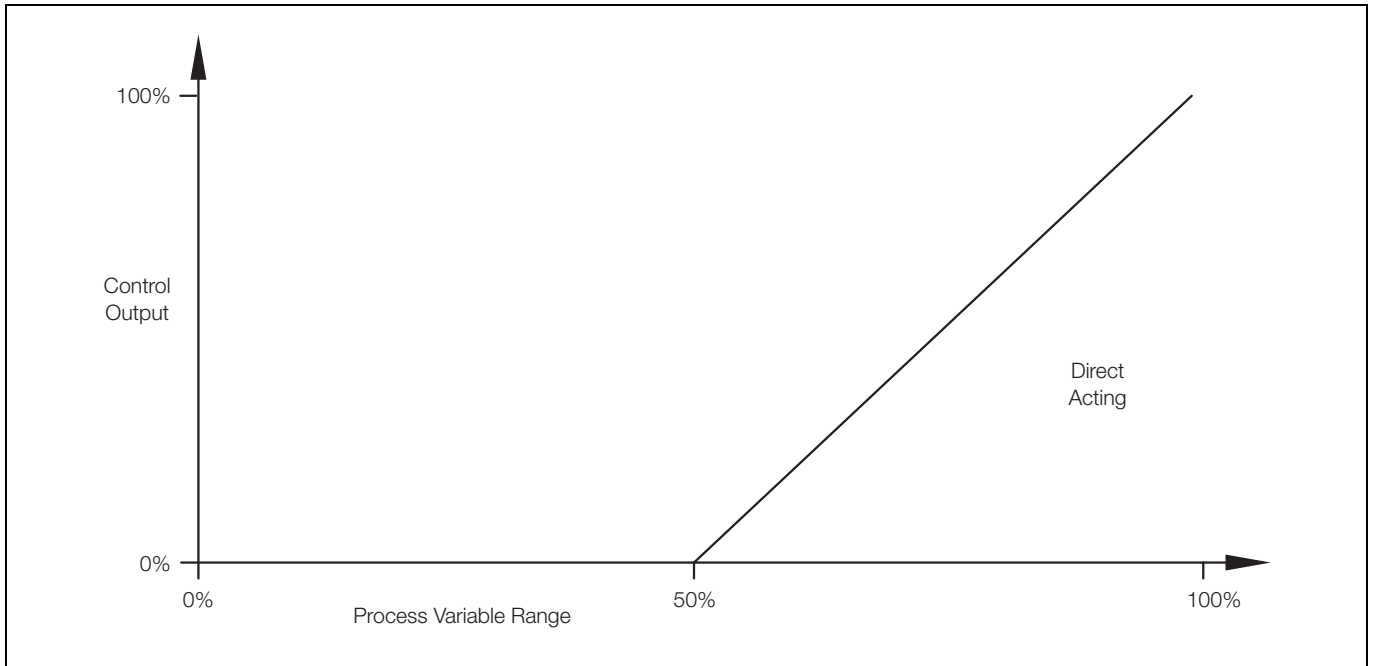
Fig. B.3 Direct Acting Single PID Control
