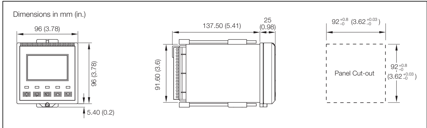
Fig. 6.4 Overall Dimensions
