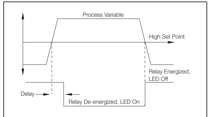
Fig. 5.5 High Failsafe Alarm with Delay but no Hysteresis
