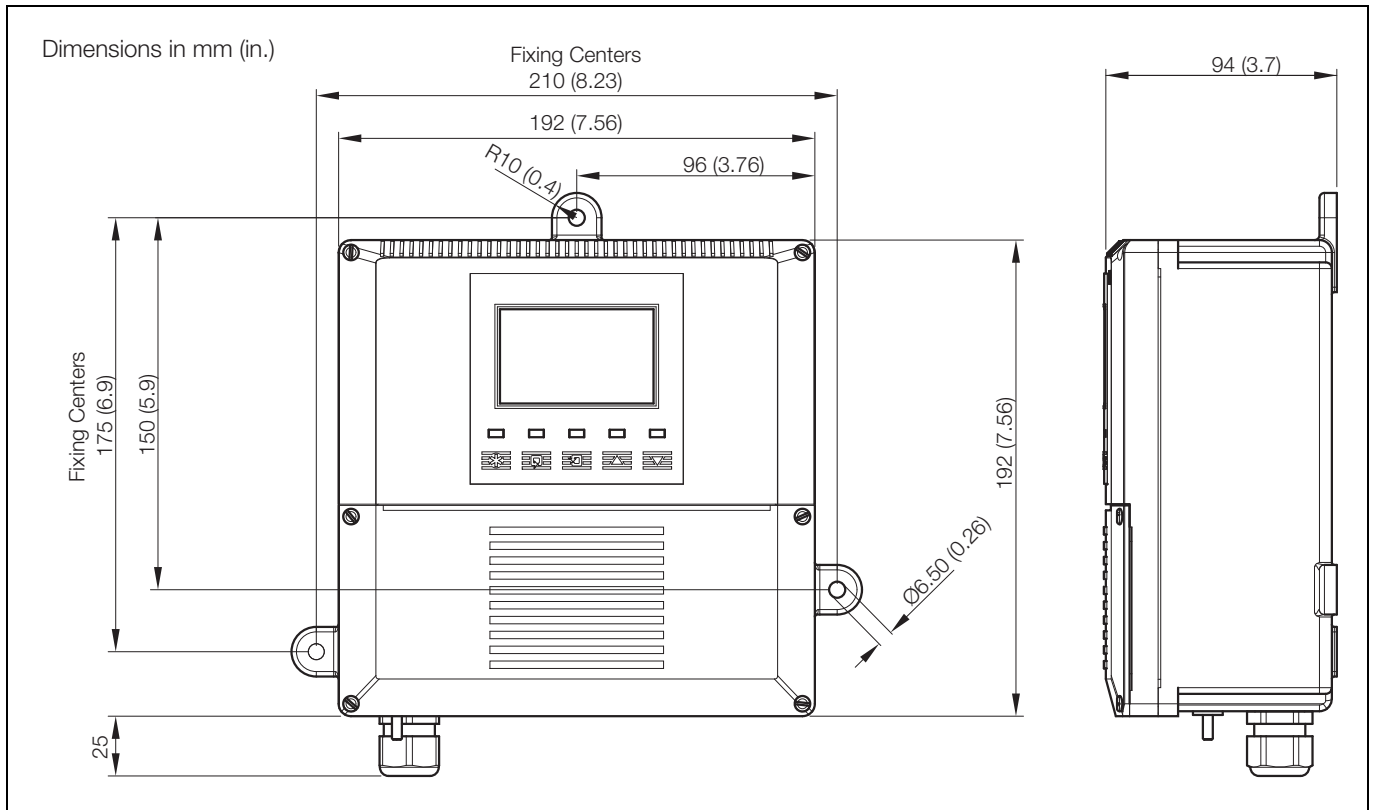
Fig. 6.2 Overall Dimensions
