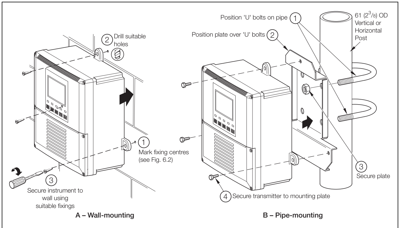
Fig. 6.3 Wall-/Pipe-mounting
