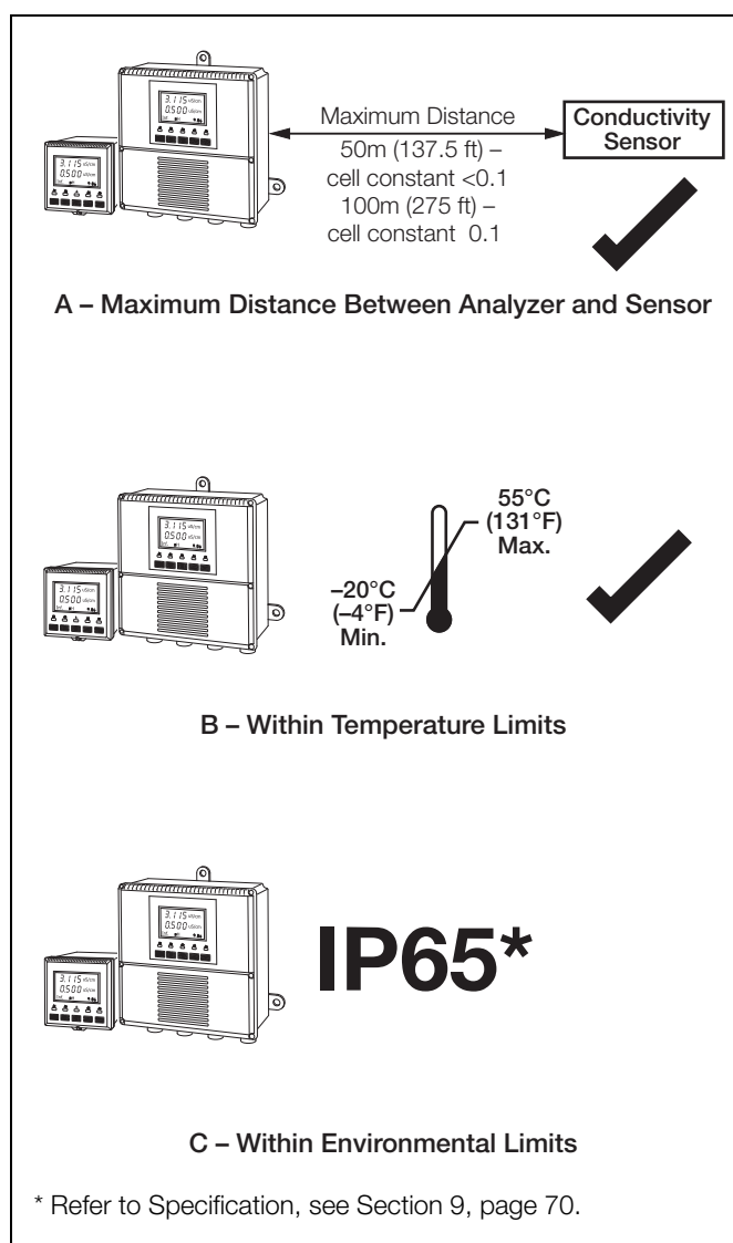
Fig. 6.1 Siting Requirements
