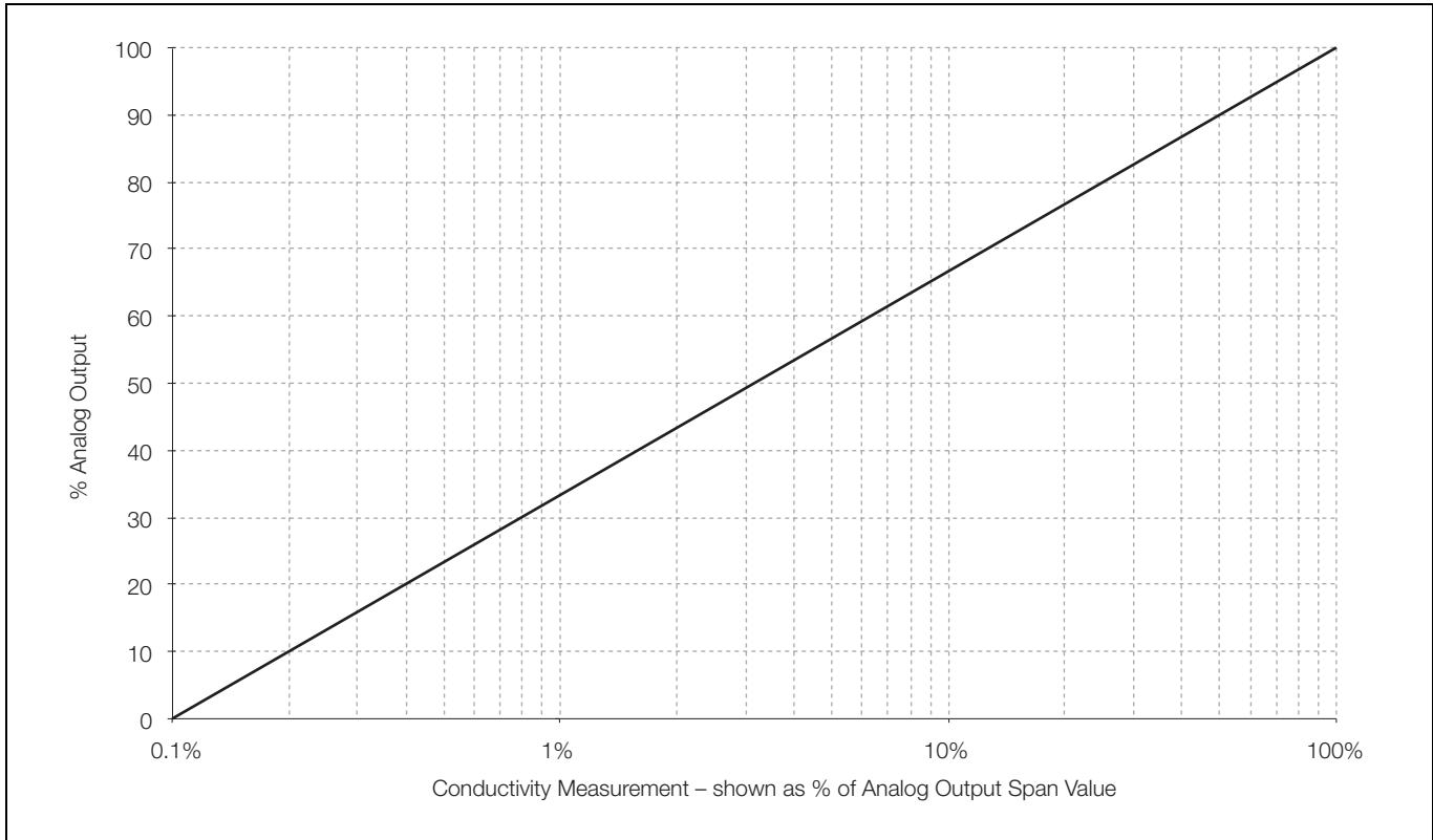
Fig. 5.8 Logarithmic Output (3-Decade)
