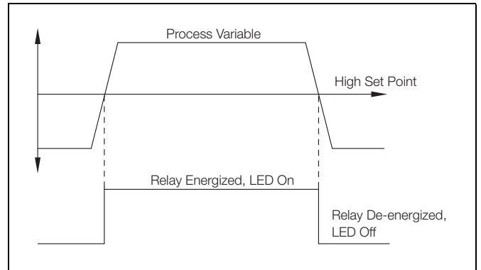
Fig. 5.4 High Non-Failsafe Alarm without Delay and Hysteresis
