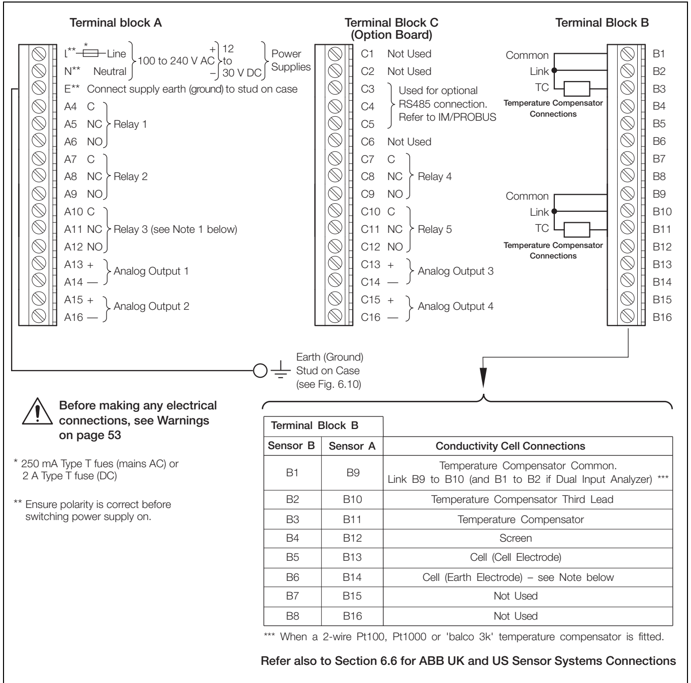
Fig. 6.11 Connections, Panel-mount Analyzers
