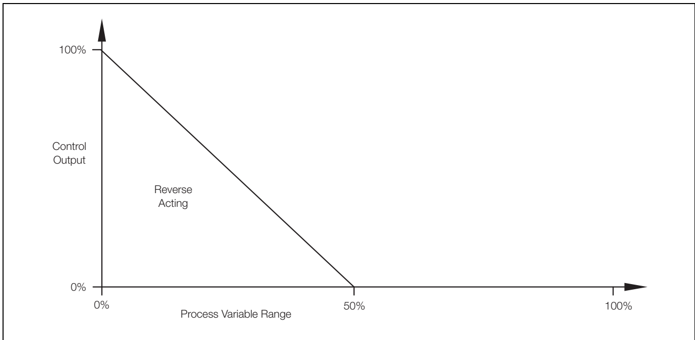
Fig. B.2 Reverse Acting Single PID Control
