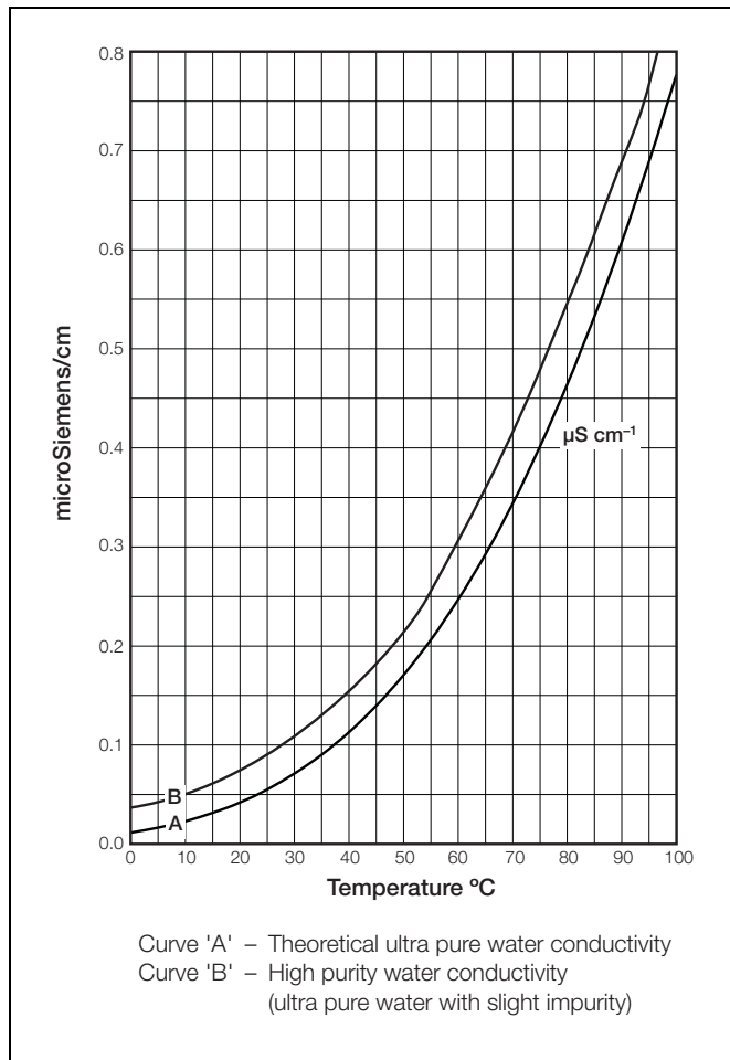
Fig. A.1 Ultra-pure Water Temperature Compensation
