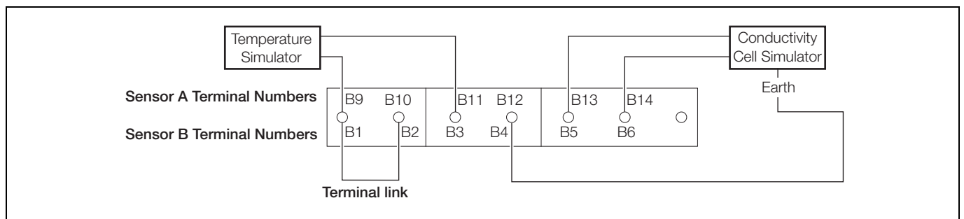
Fig. 7.1 Analyzer Terminal Links and Decade Resistance Box Connections
