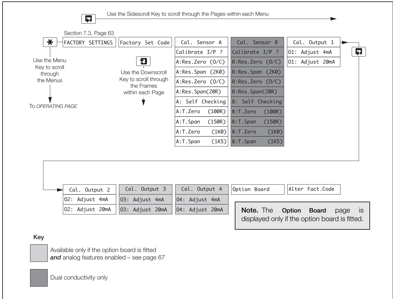
Fig. 7.2 Overall Factory Settings Chart
