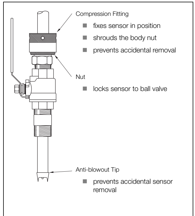
AP304 and AP305 Anti-blowout Tip and Hand-compression Fitting Safety Features
