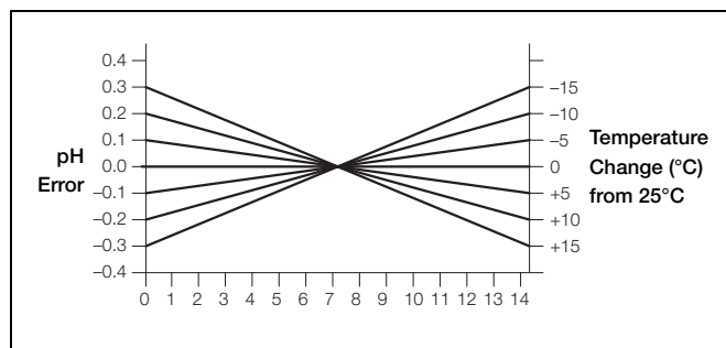
Temperature Compensation
