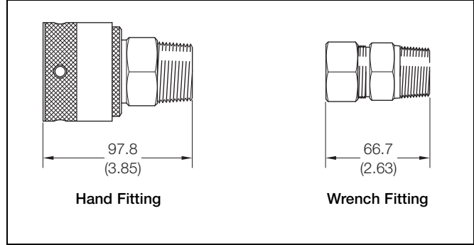
AP304/5 Compression Fittings
