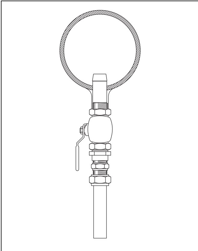
AP304 Hot-tap Sensor – Typical Installation
