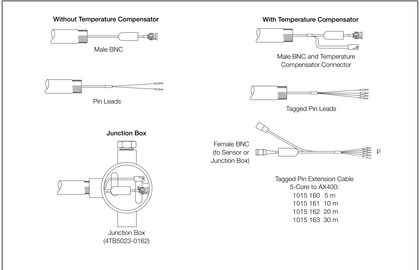
Sensor Cables and Junction Box Wiring
