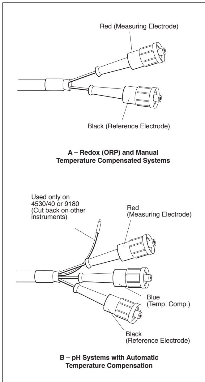
Fig. 2.3 Cable Termination - Electrode Connections
