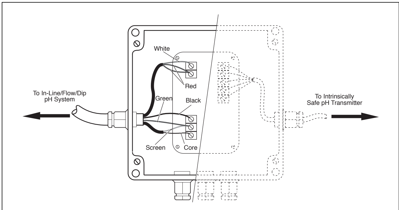
Fig. 4.2 Junction Box Electrode Connections
