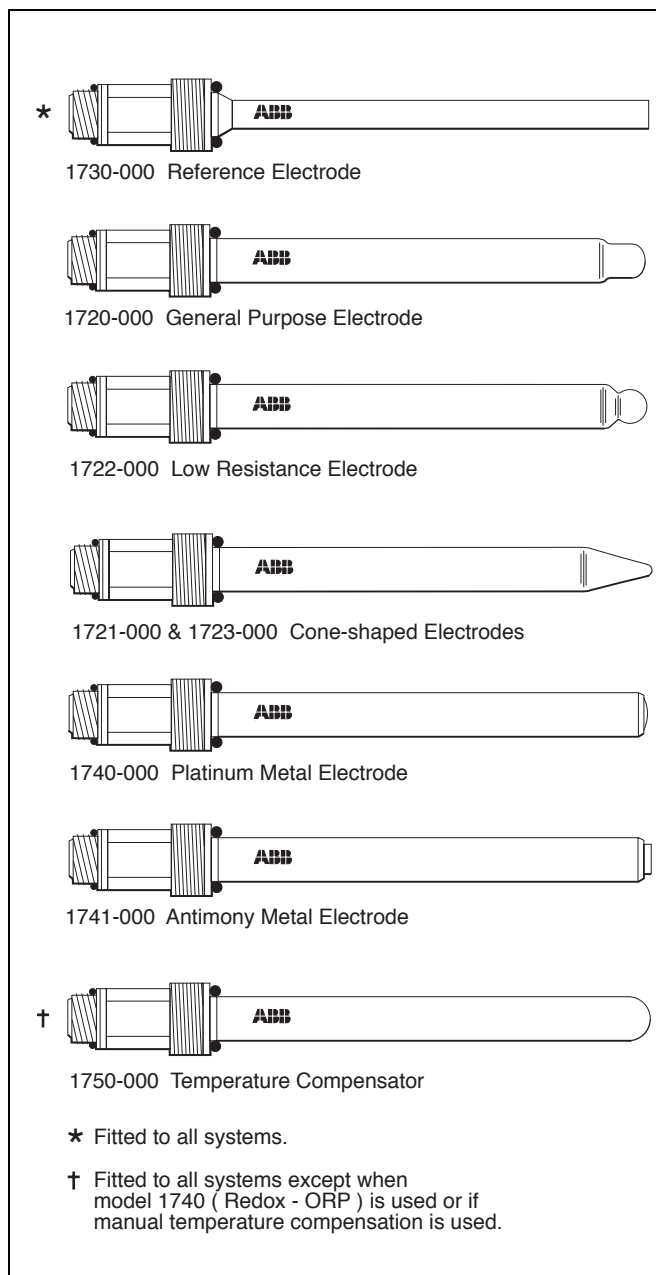
Fig. 2.2 Electrode Models
