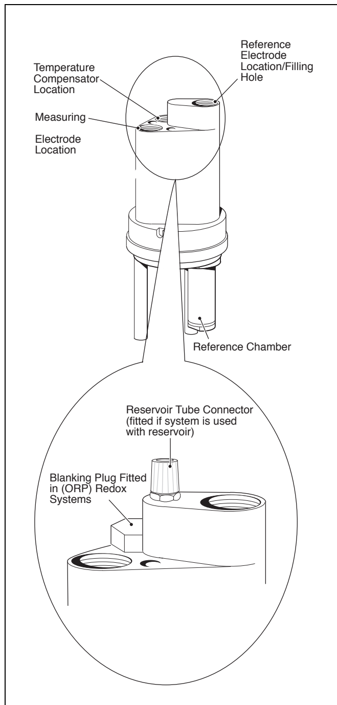
Fig. 3.10 Location of Blanking Plug and Reservoir Tube Connector
