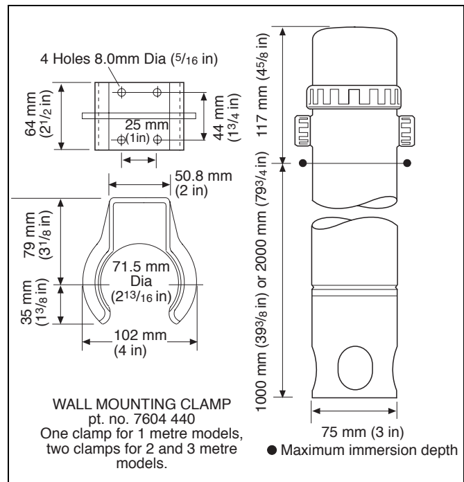
Fig. 3.4 Mounting, Types 7654, 7655, 7656, 7664 and 7665
