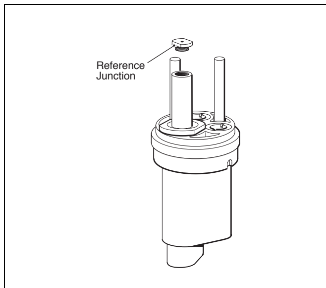
Fig. 3.8 Sealed Types (Electrodes and Temperature Compensator Omitted for Clarity)
