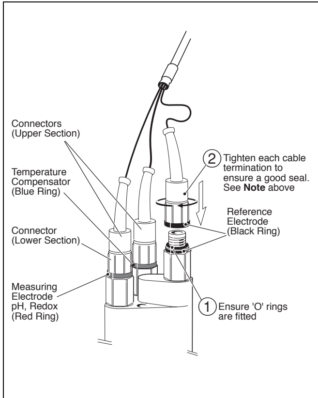
Fig. 3.11 Fitting the Electrode Connectors
