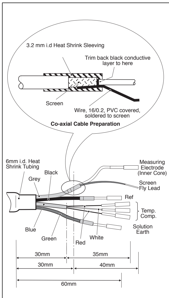
Fig. 4.3 Cable Termination
