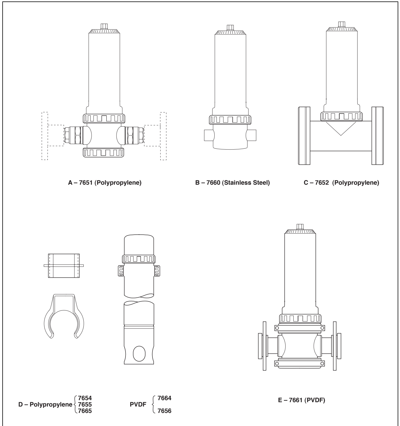
Fig. 2.1 System Types
