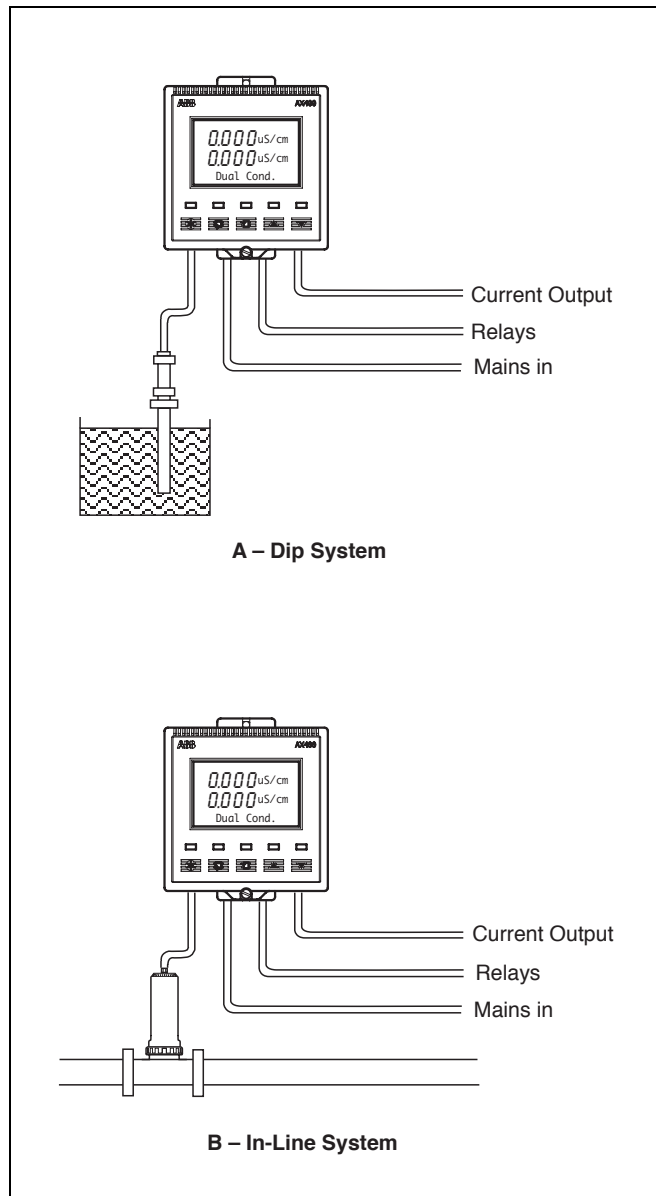
Fig. 1.1 Schematic Diagrams
