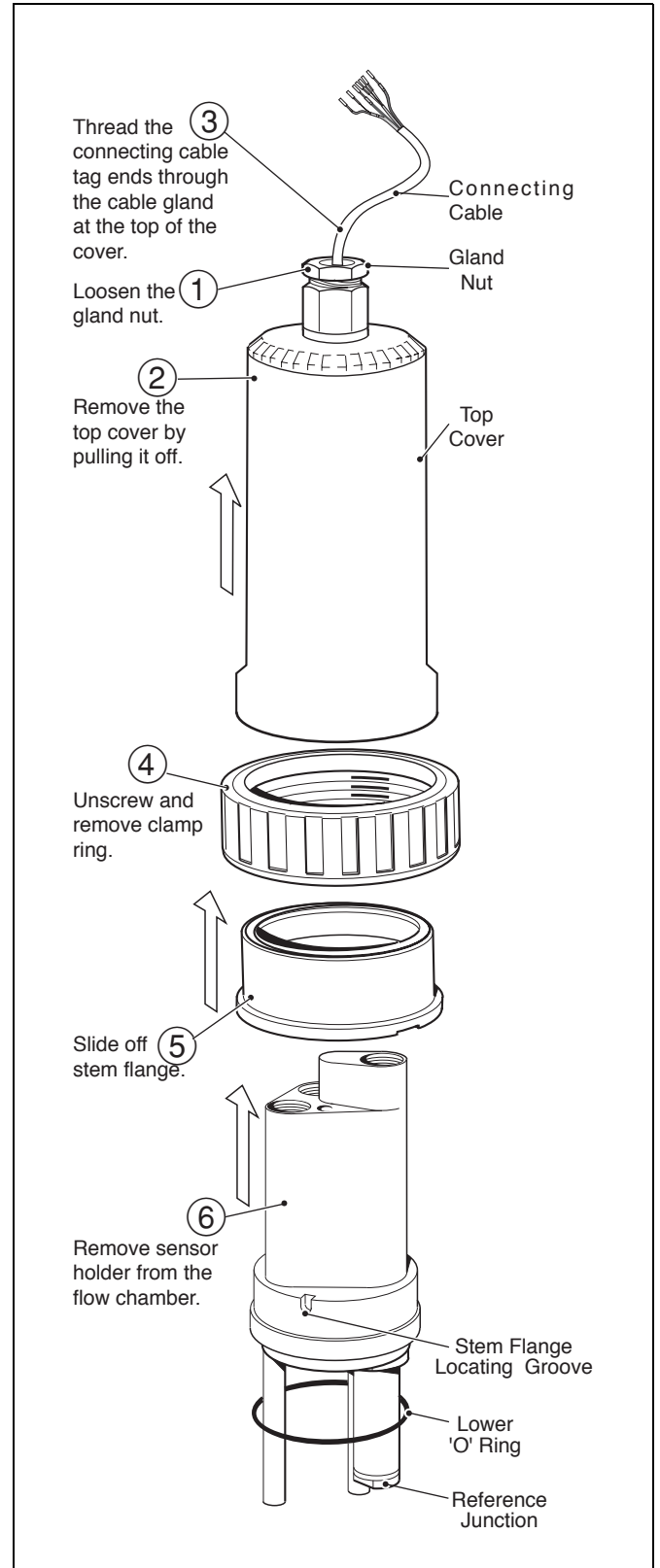
Fig. 3.6 Access to Sensor Holder for Flow and In-line Systems - Models 7651, 7652, 7660 and 7661
