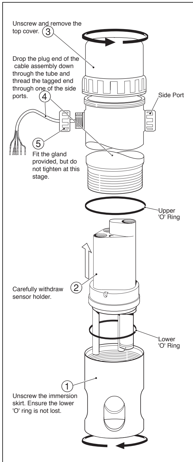
Fig. 3.7 Access to Sensor Holder for Dip Systems - Models 7654, 7655, 7656, 7664 & 7665
