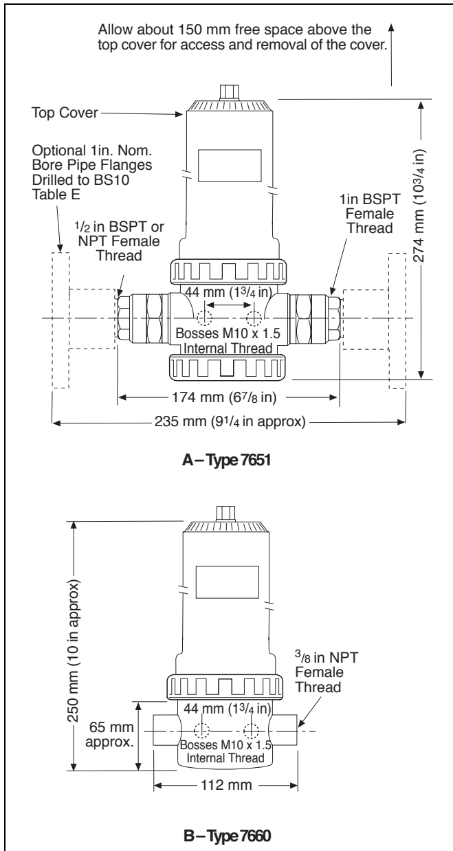
Fig. 3.2 Mounting, Types 7651 and 7660
