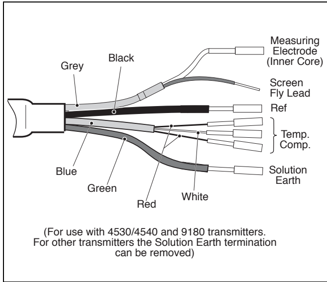
Fig. 4.1 System Connections
