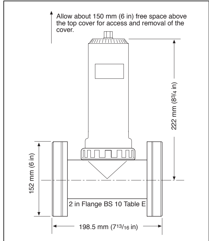
Fig. 3.3 Mounting, Type 7652
