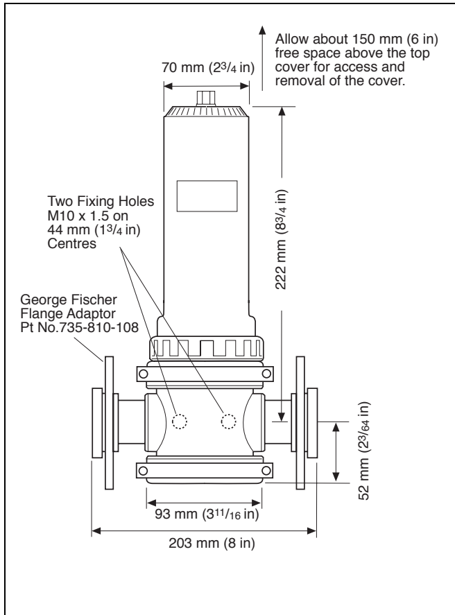
Fig. 3.5 Mounting, Type 7661
