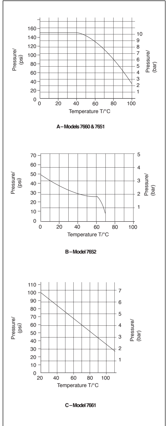
Fig. 3.1 Operating Temperatures and Pressures
