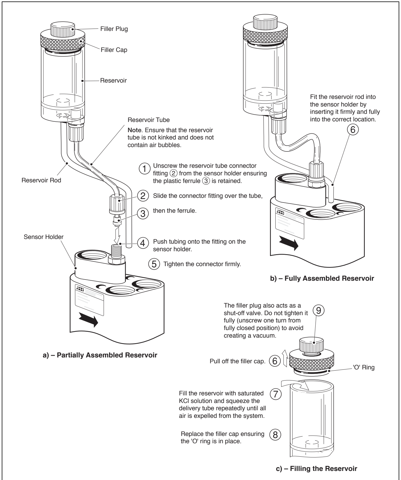
Fig. 3.12 Fitting and Filling the Reservoir (Electrodes and Temperature Compensator Omitted for Clarity)
