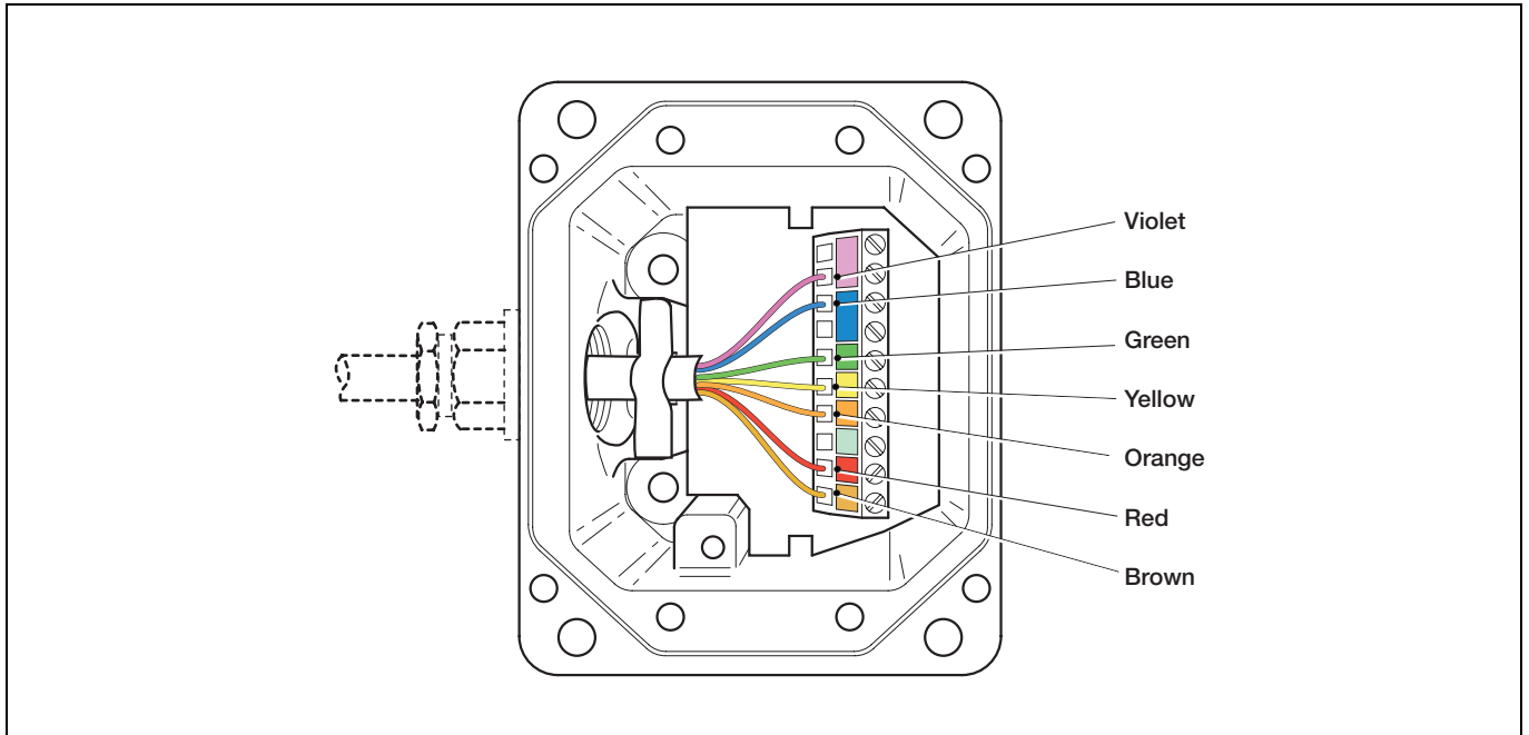
Fig. 1.1 Sensor Terminal Box Connections (Remote Version)
