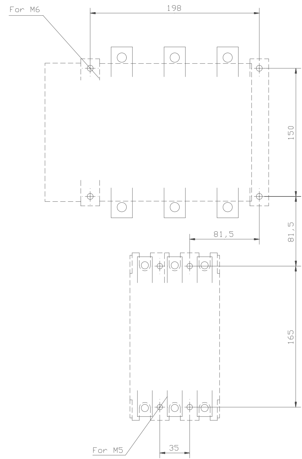
Drilling plan Borrplan
