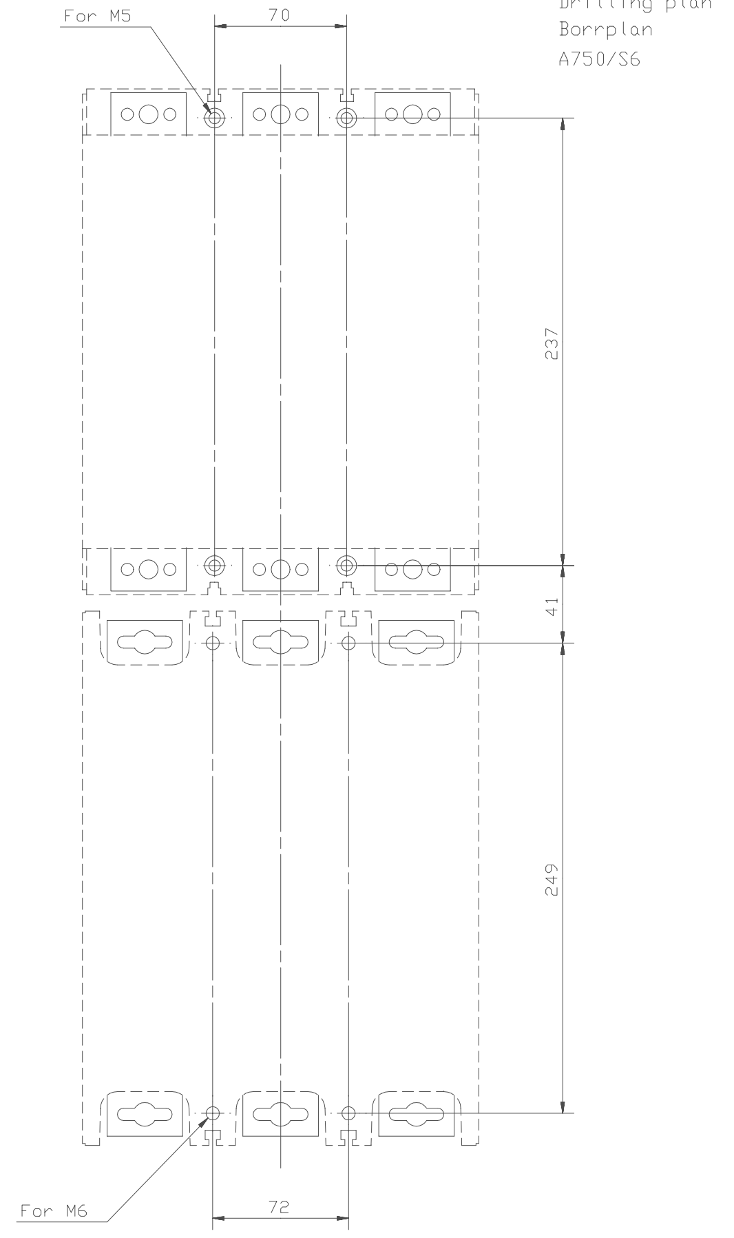
Connection bars between contactor and MCCB A460-A750/S6
