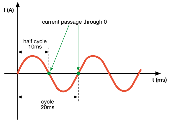
Figure 7 Alternating current
