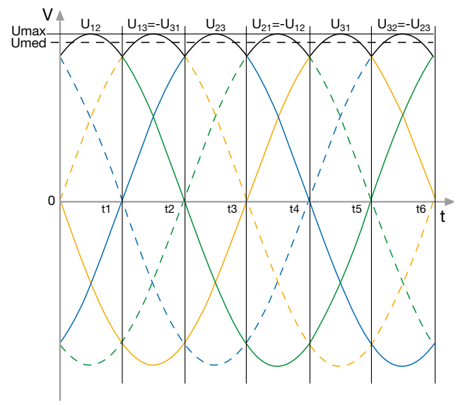
The continuous lines represent the three sine curves of the line-to-line voltages ( U_{12} ; U_{23} ; U_{31} ), whereas the dotted lines represent the sine curves of the same voltages but reversed ( U_{13} = -U_{31} ; U_{21} = -U_{12} ; U_{32} = -U_{23} ).
