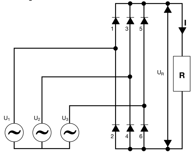
In this diagram it is possible to identify the three forward diodes (1,3,5) having the cathodes connected in common and the three backward diodes (2,4,6) which instead have the anodes connected in common.
