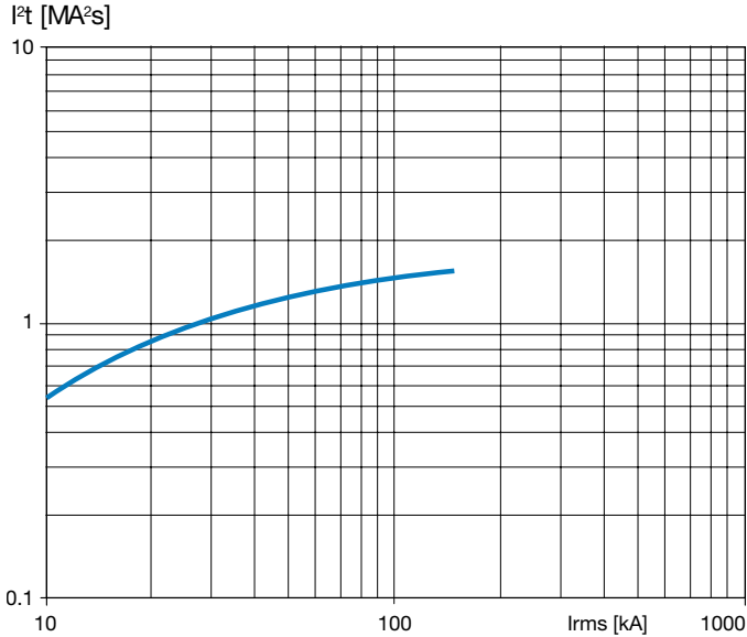
Figure 20: Specific let-through energy curve
