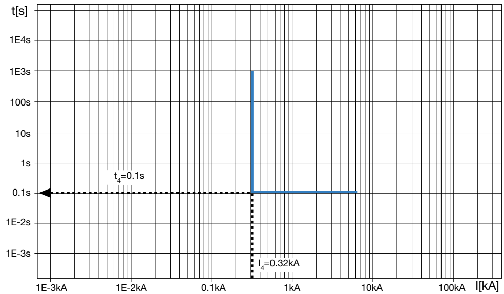
Figure 19: Function G at t = K
