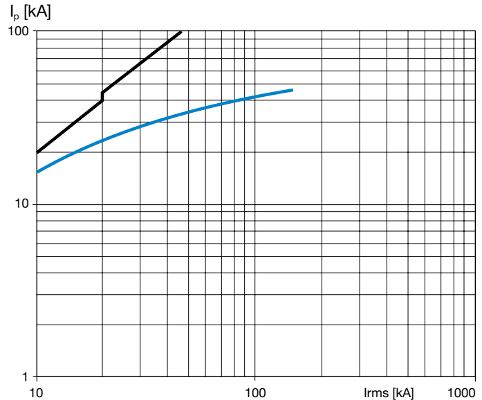
Figure 21: Limitation curve
