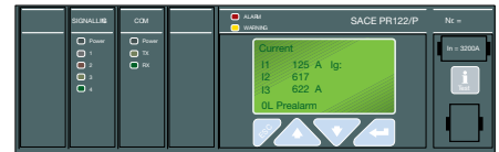
Trip unit front
