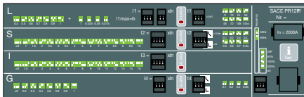
Trip unit front
