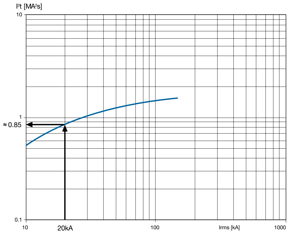
Figure 22: Specific let-through energy curves @ 480V
