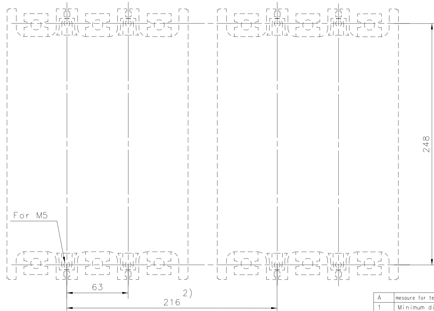
Drilling Plan Borrplan
