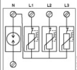
Operating diagram
