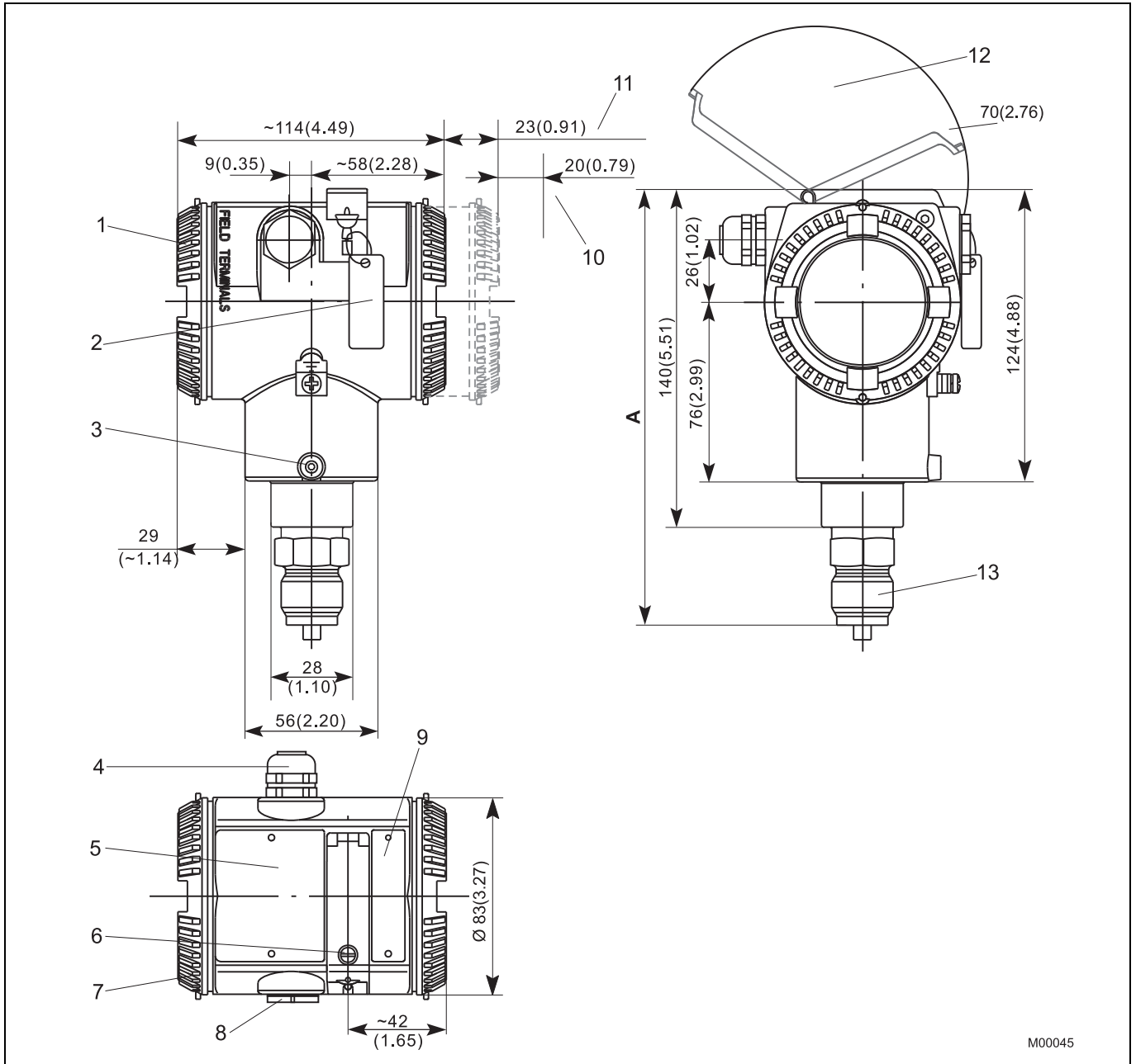
Fig. 24: Dimensions in mm (inch)
