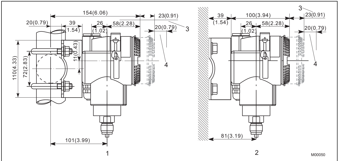
Fig. 29: Dimensions in mm (inch)
