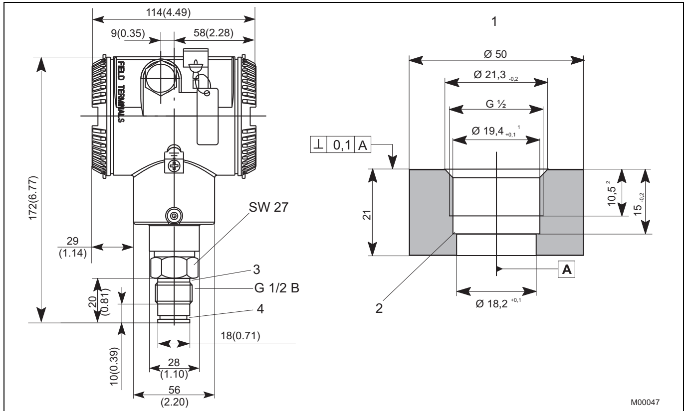
Fig. 26: Dimensions in mm (inch)
