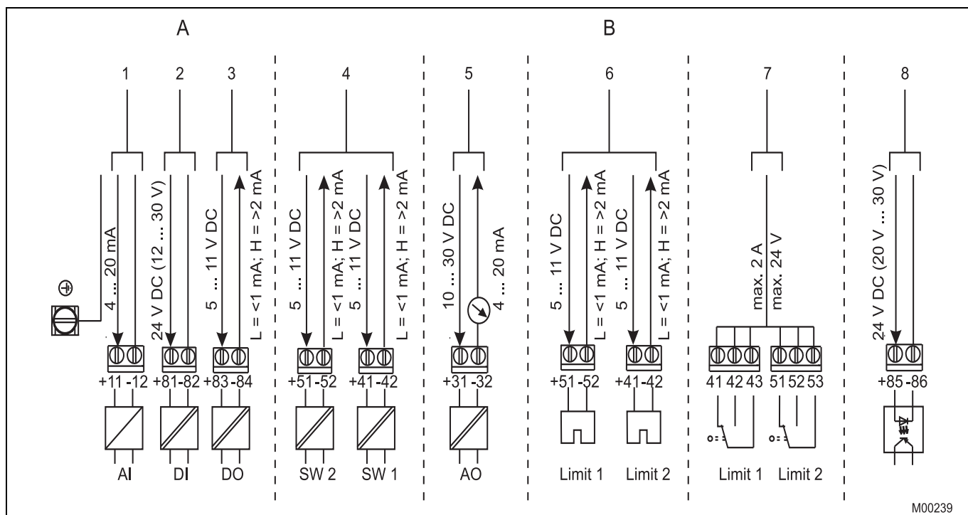
Fig. 8: Pin configuration
