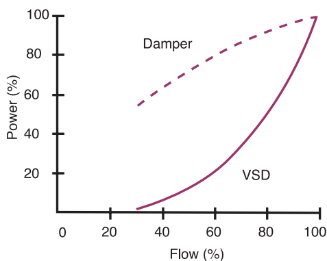
Fig. 1: Graph showing fan power requirements for damper and VSD.
