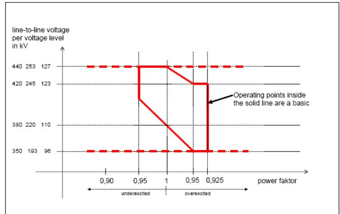
Fig. 2. Grid Code requirements: reactive power provision.
