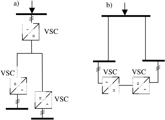
Figure 7. Examples of topologies for City Infeed using VSC based HVDC. Example b) gives increased overall reliability of supply. In both a) and b) the VSC will give increased voltage performance with reactive power control in the HVDC converters. Alternative b) is topologically equivalent to closing an open loop circuit, which with HVDC gives an extended system without increasing the short circuit power.
