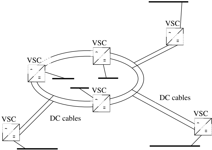
Figure 8: Vision of a modern multi-terminal HVDC network with VSC converters and extruded cables. This could be a new system or an expansion of an existing city network. In this example power is fed from the transmission grid and distributed through a dc-cable ring to inverter stations.
