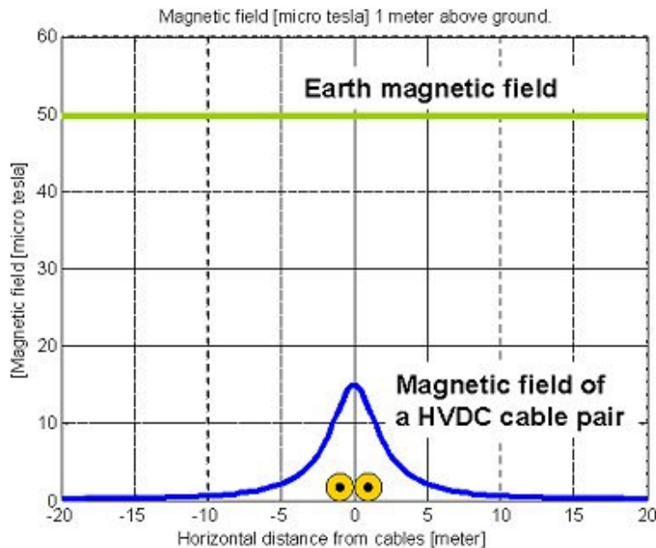
Figure 3. The static magnetic field of a pair of HVDC cables (300 MW) buried 1 meter below the surface and calculated at a level of 1 meter above the surface. In addition the earth magnetic field is shown.
