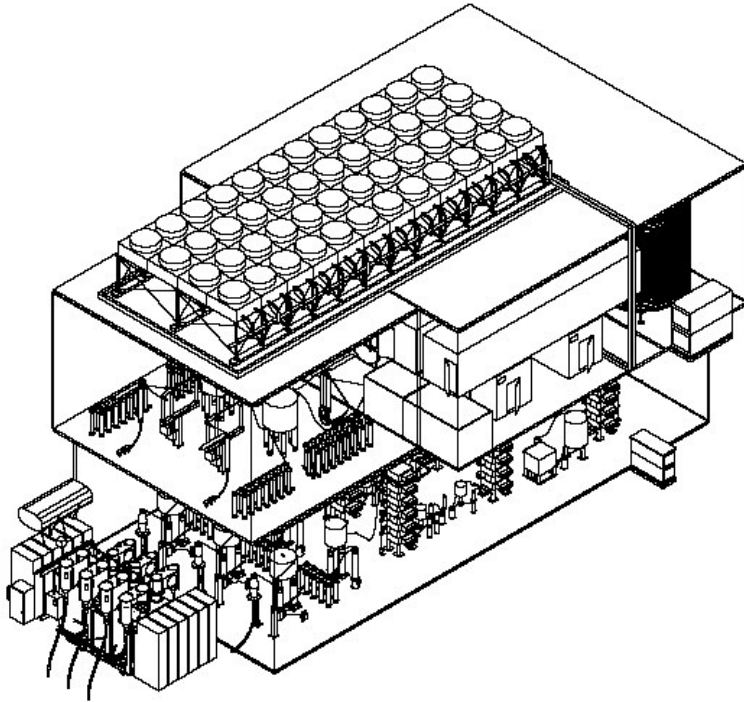
Figure 2. Possible layout of compact VSC station for 500 MW. Dimensions in this configuration are 48 x 25 x 27 m (L x W x H). Ground floor: Transformer and AC-side filters. First floor: Phase reactors, converter valves, control and cooling equipment, DC-side filters and cable terminations. Second floor: Cooling fans, which may be omitted if a nearby river or other water is available for cooling.
