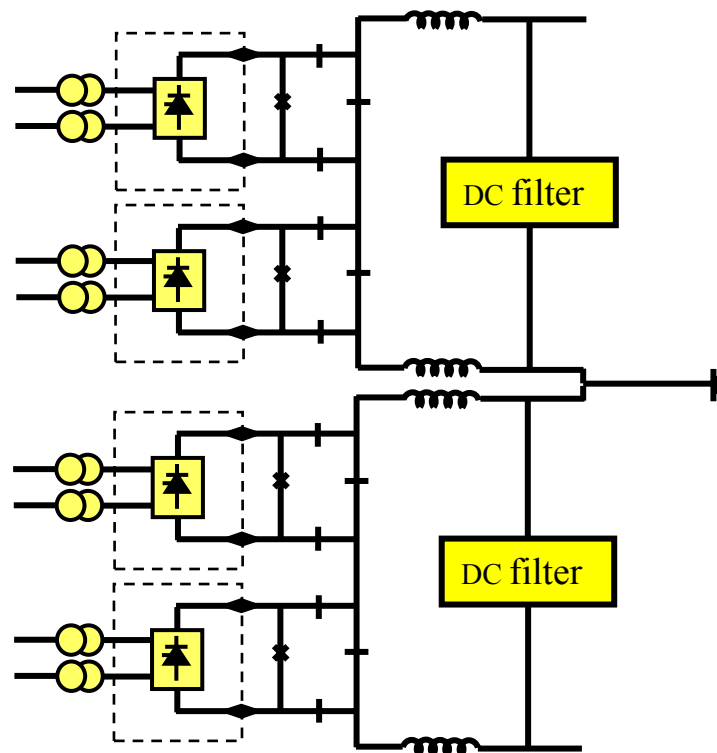
Fig. 3. Overview single line diagram of Xiangjiaba – Shanghai \pm 800 kV DC Transmission Project, clearly showing the two-series converters per pole.
