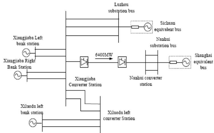
Fig. 2. Power system around the Xiangjiaba – Shanghai \pm 800 kV DC Transmission Project
