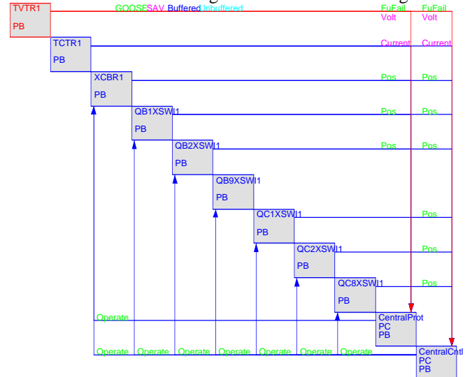
Figure 4 – Central solution with 1 bay connected
