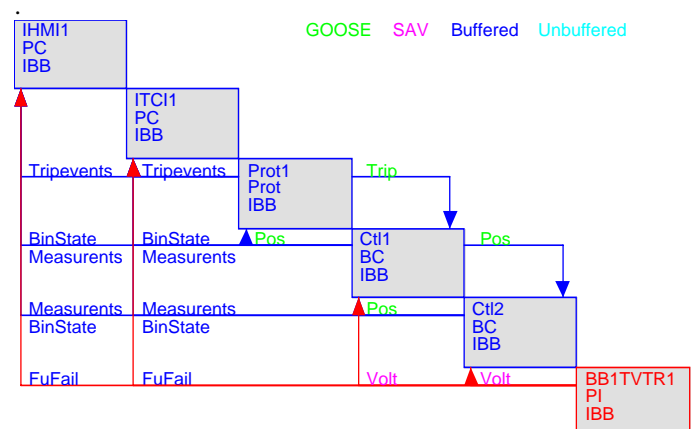
Figure 5 – One conventional bay exchanging Interbay data and receiving samples from busbar VT
