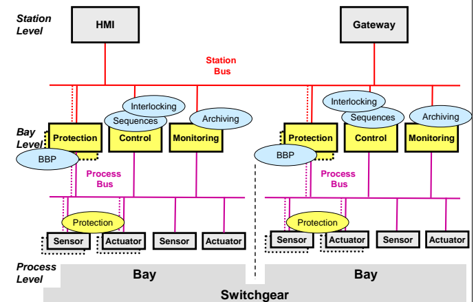
Figure 3 – Toward a totally decentralized SA system (schematic)
