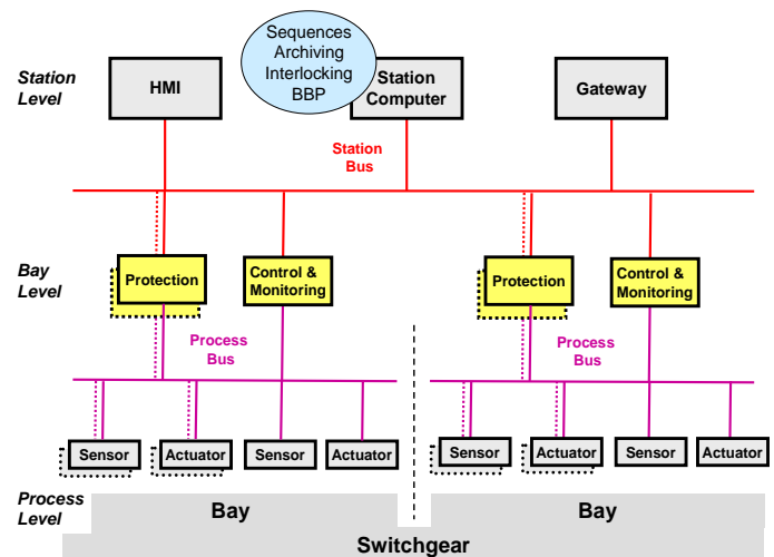
Figure 1 – Common structure and function allocation in SA systems
