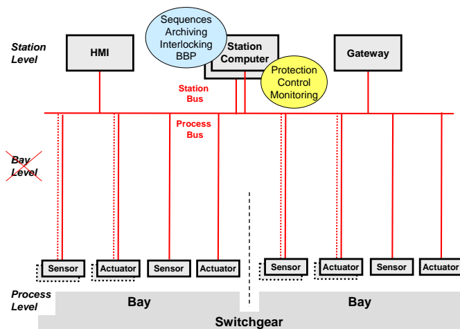
Figure 2 – Totally centralized SA system with sensors and actuators
