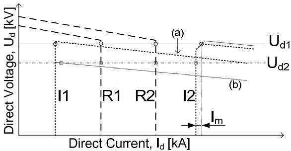
Fig. 2. Voltage - Current characteristics for the parallel converters in Fig. 1.
