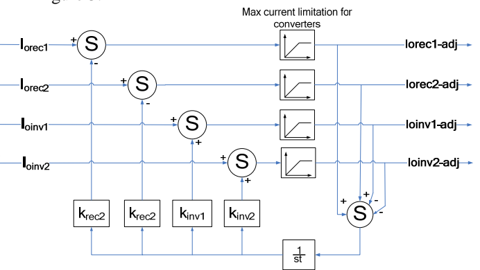
Fig. 3. Block diagram for a four terminal current order calculation.
