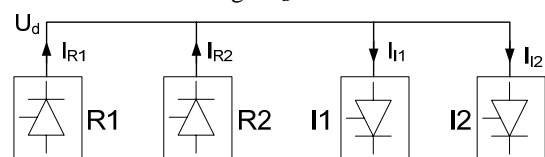
Fig. 1. Multi-terminal HVDC system with two rectifiers and two inverters.
