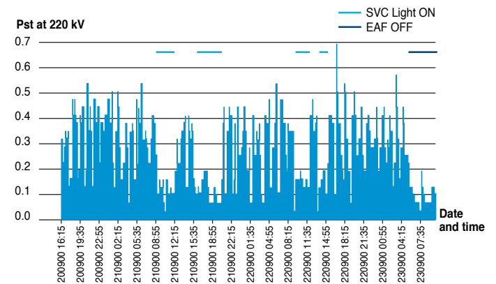
Flicker recordings at the 220 kV PCC with and without the SVC Light in operation.
