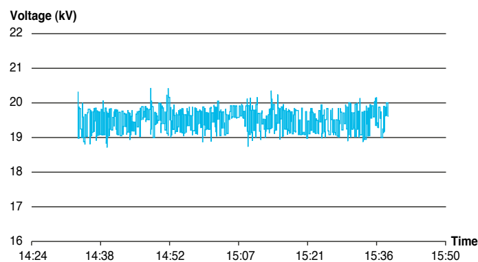
EAF bus voltage without and with SVC Light.
