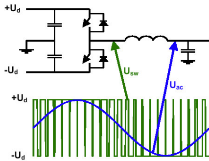
Figure 1 PWM, Pulse With Modulation
