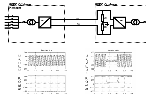
Figure 3 HVDC Light ® with chopper solution
