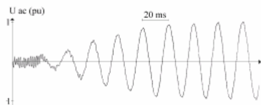
Figure 4 AC voltage at start-up of an isolated network (measurements from the Hällsjö project)
