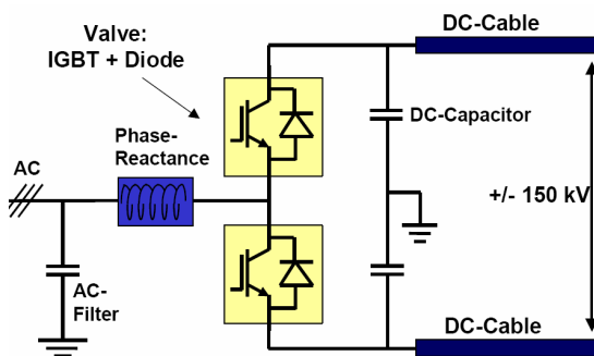
Figure 2 HVDC Light principles
