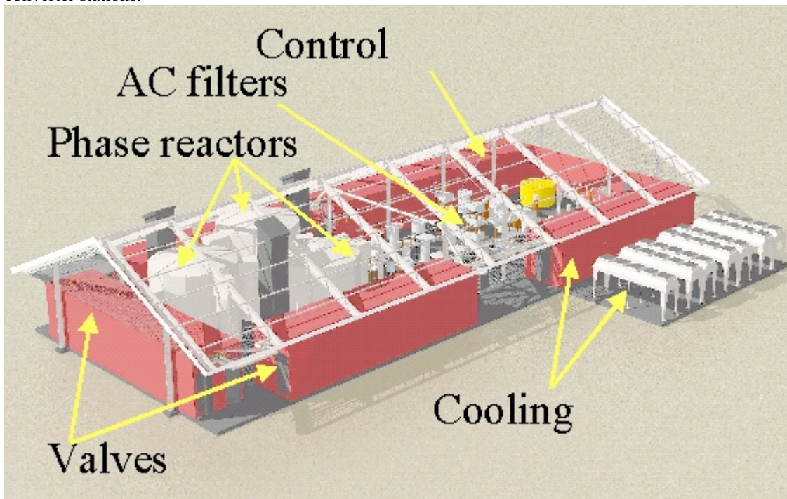
Fig. 3. HVDC Light converter
