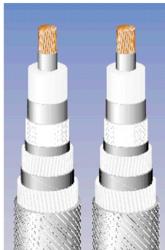
Fig. 4 shows 10 – 600 MW deep sea HVDC Light cable
