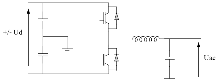
Fig. 1 shows one phase of a VSC converter using PWM
