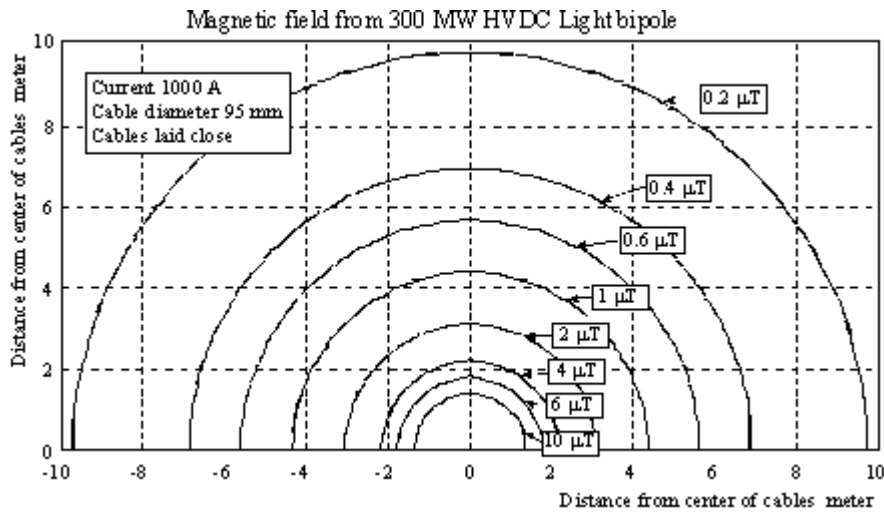
Fig. 6 shows iso-Tesla curves for 300 MW HVDC Light submarine and land cables.
