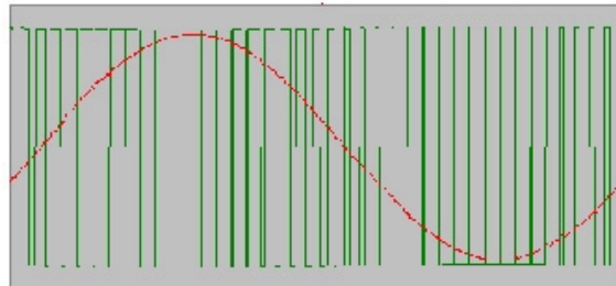
Fig. 1 shows one phase of a VSC converter using PWM
