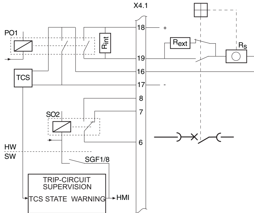
Fig. 5.1.5.-1 Connecting the trip-circuit supervision using two external contacts and the external resistor in the trip circuit
