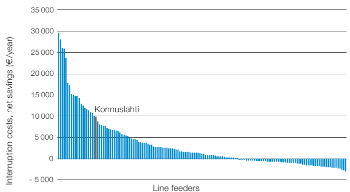
The potential profitability of reclosers as per line feeder.
