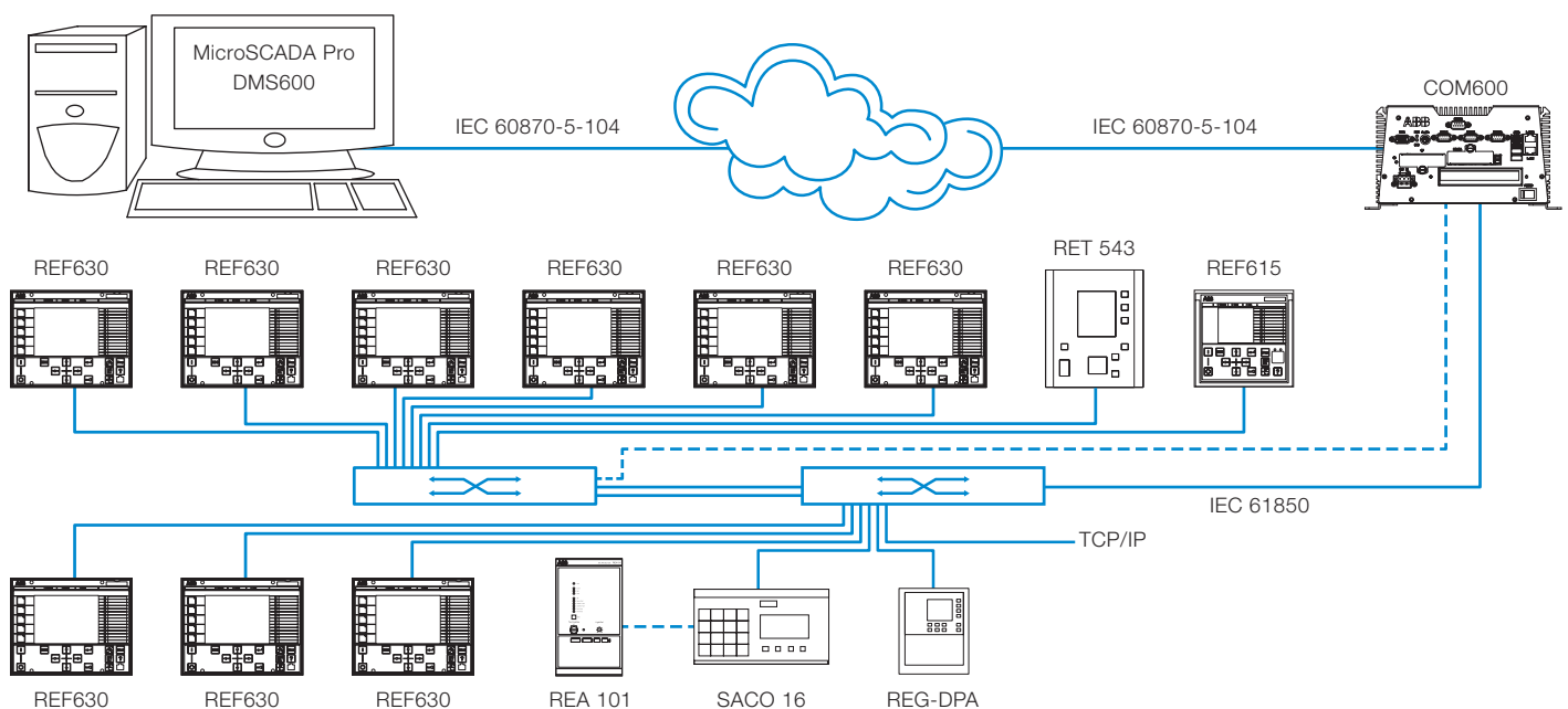
The IEC 61850 substation automation bus solution and its connection to the ABB's MicroSCADA Pro and DMS 600 of the Pellesmäki substation.
