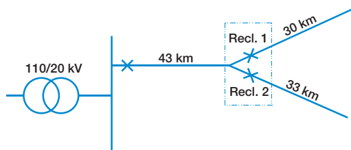
Location of the Konnuslahti recloser station on the line feeder.
