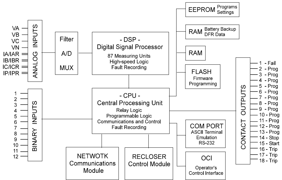
Main Board Block Diagram
