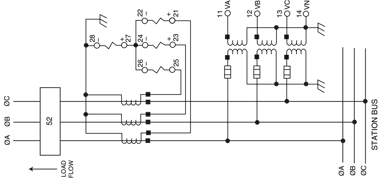
Figure 4. Typical Connections
