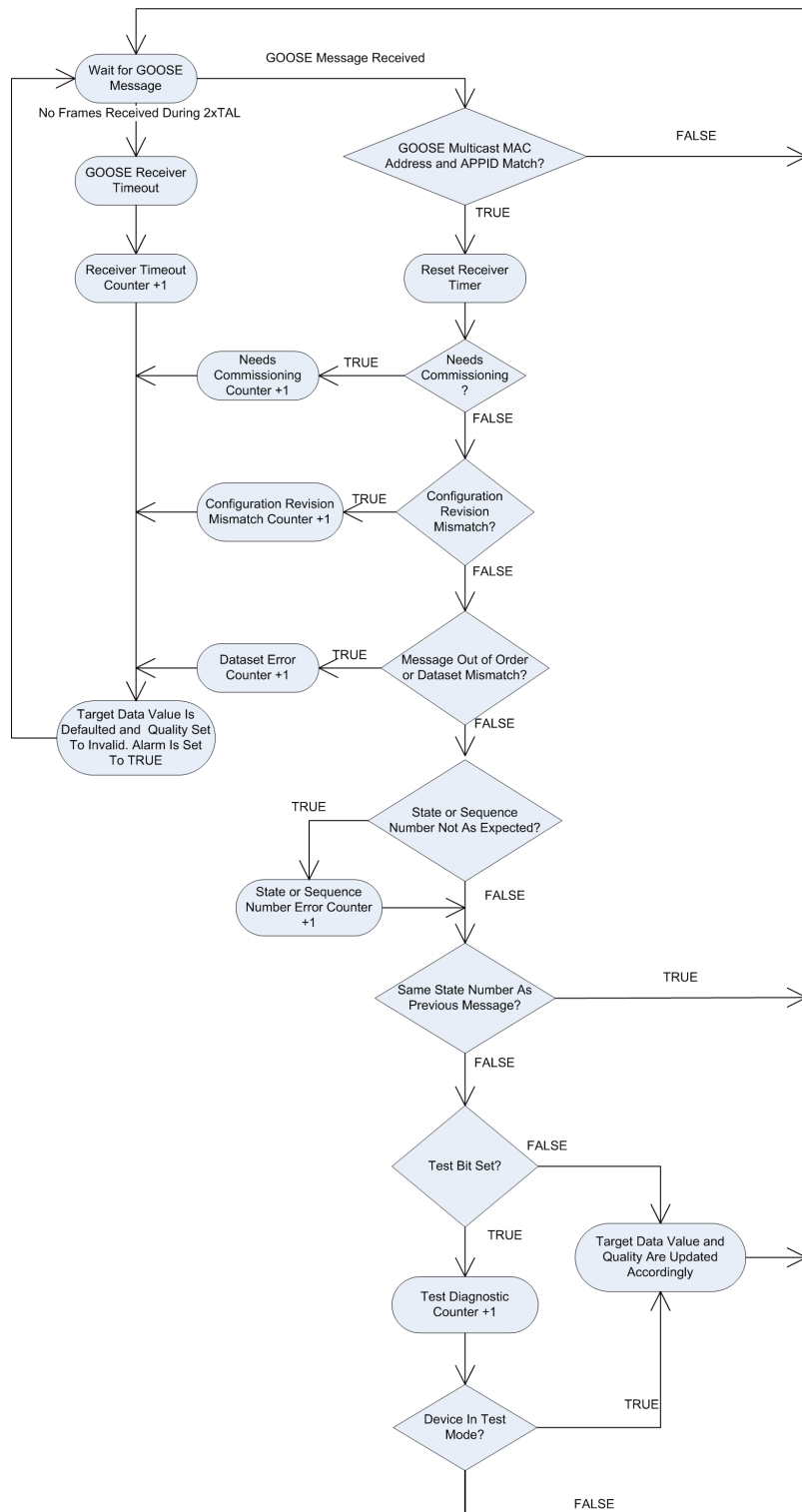
Figure 25: Receiving GOOSE data in 615 series IEDs
