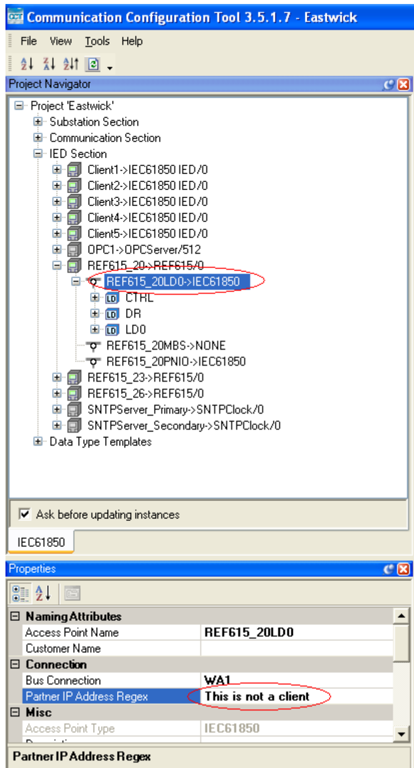
Figure 28: Defining server IEDs in CCT600
