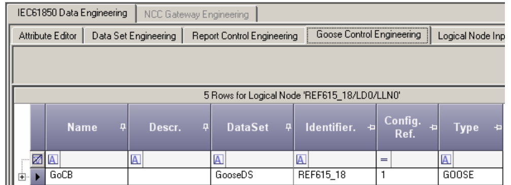
Figure 12: GOOSE control block basic properties
