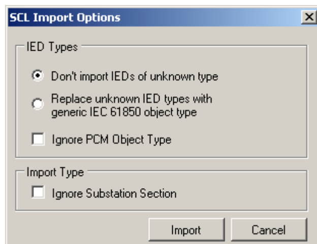
Figure 22: SCL import options in PCM600
