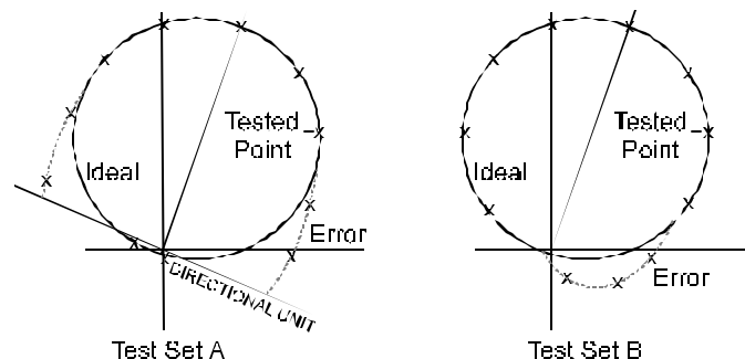
Figure 2 - Apparent Impedance Characteristic Error Due To Pulse Testing
