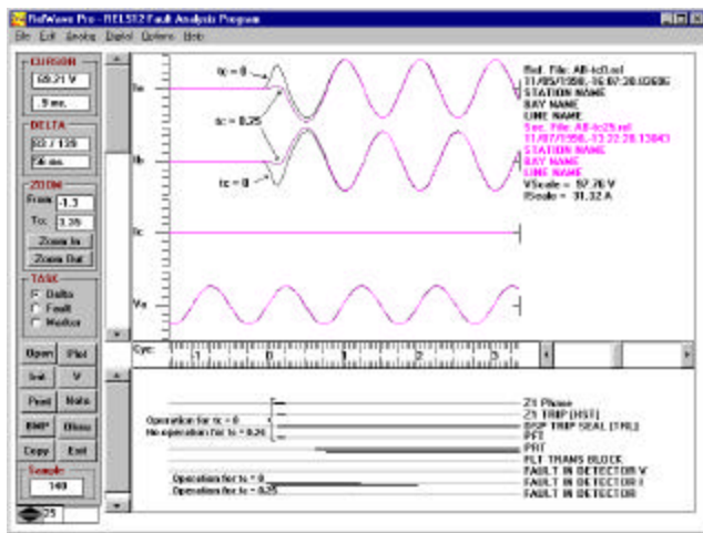
Figure 3 - Tests Using Time Constants of t_c = 0.0 and t_c = 0.25 Cycle
