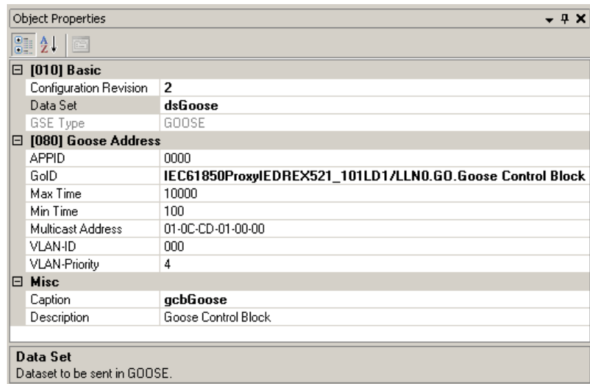
Figure 3.4.6-4 GOOSE Control Block properties
