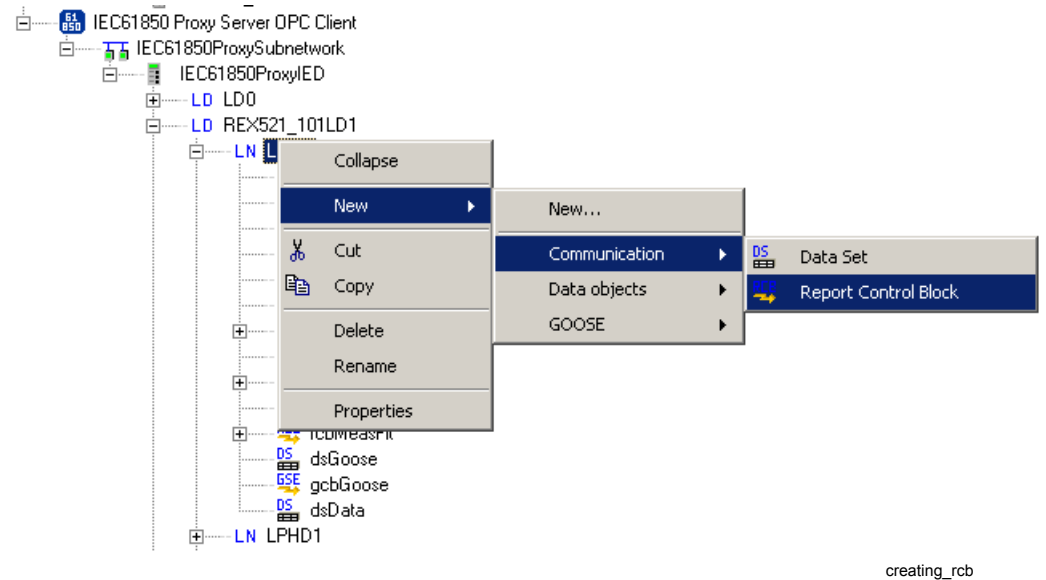
Figure 3.4.4-2 Creating a new report control block
