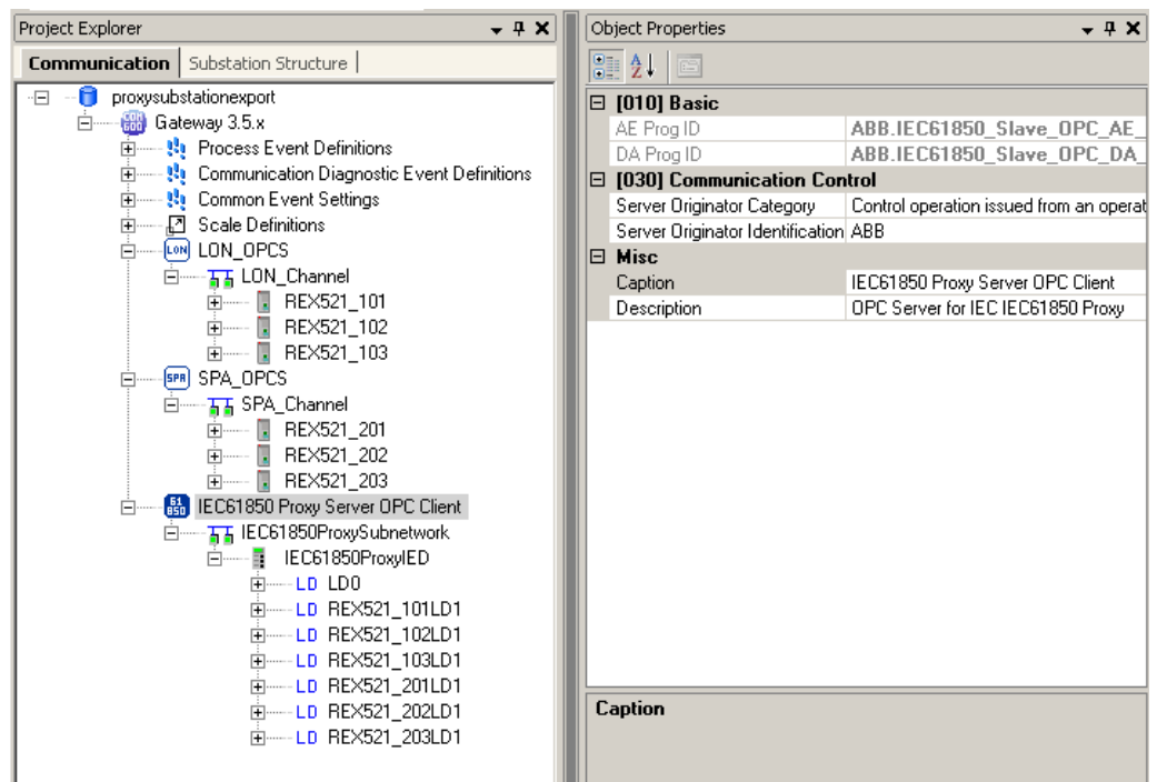
Figure 3.2-1 Example view of SAB600 communication structure
