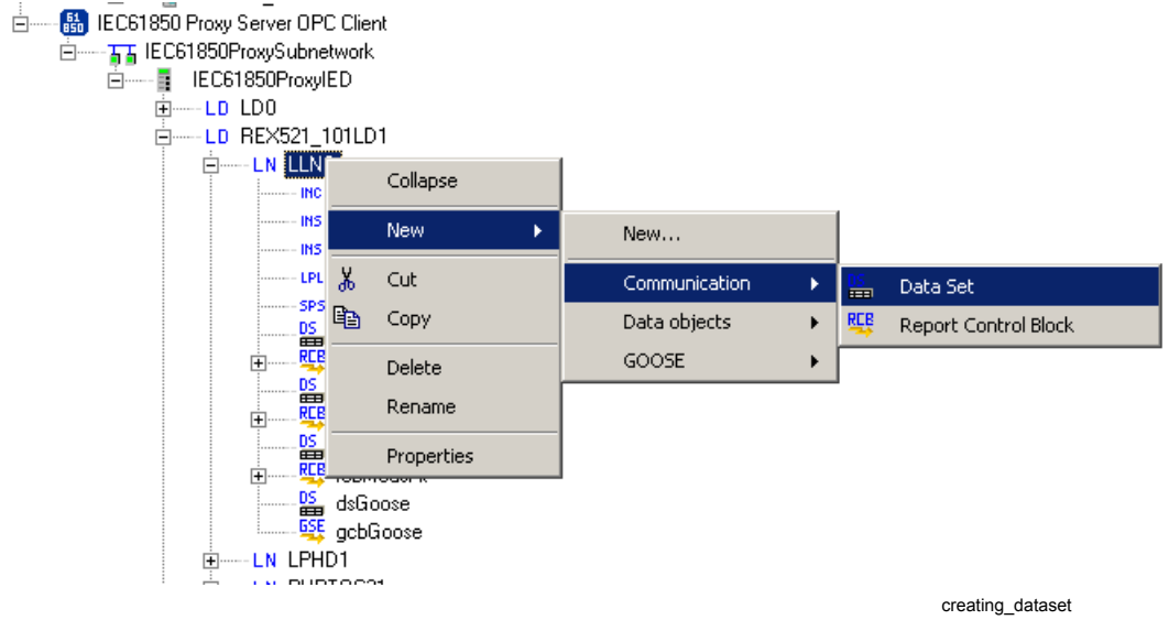
Figure 3.4.4-1 Creating a new data set
