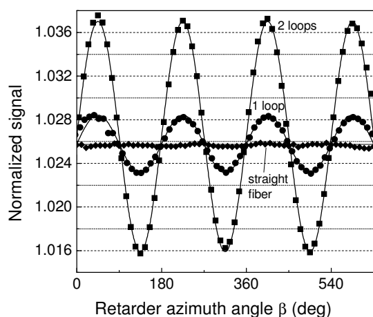
Fig. 4 Signal vs. azimuth angle of the 103^\circ -retarder for straight sensing fiber and fiber coiled to one and two loops (experiment and theory).
