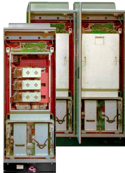
Converter module with and without cover plate
