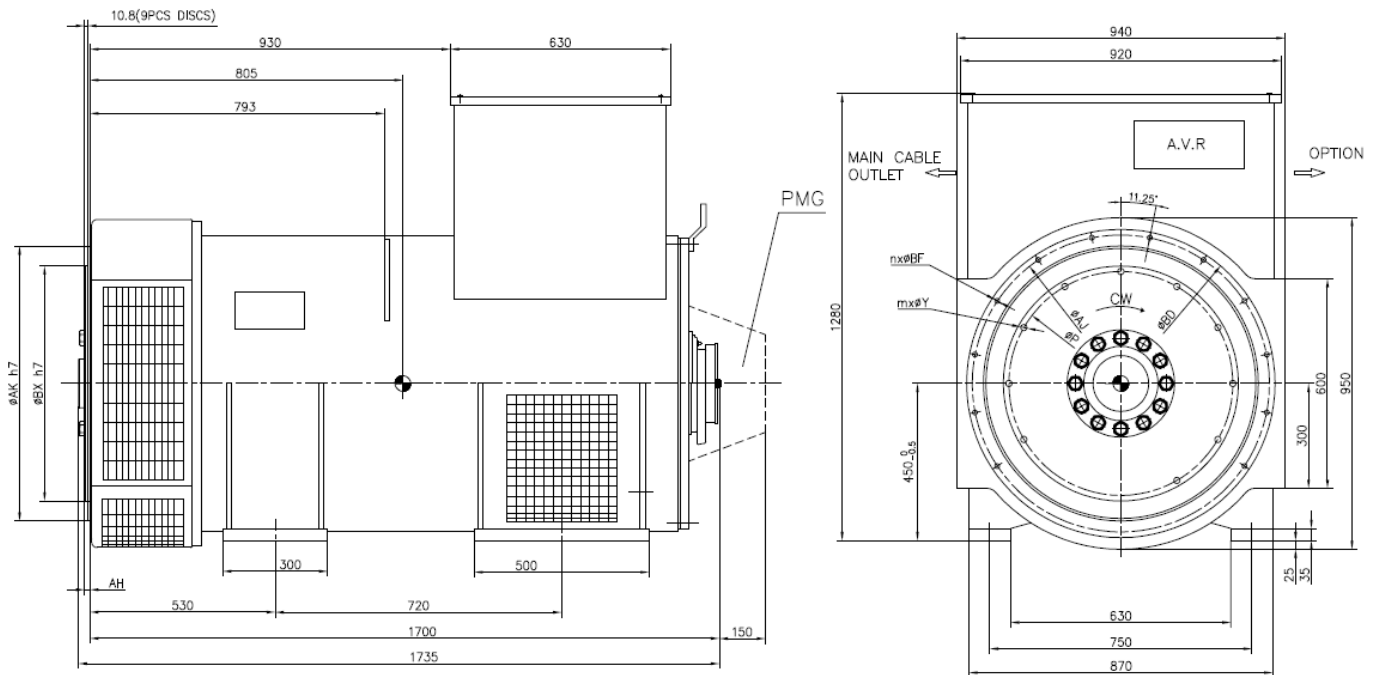
Flange dimensions
