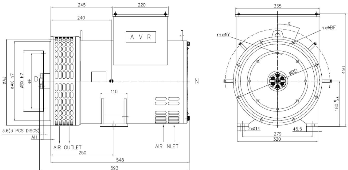
Flange dimensions
