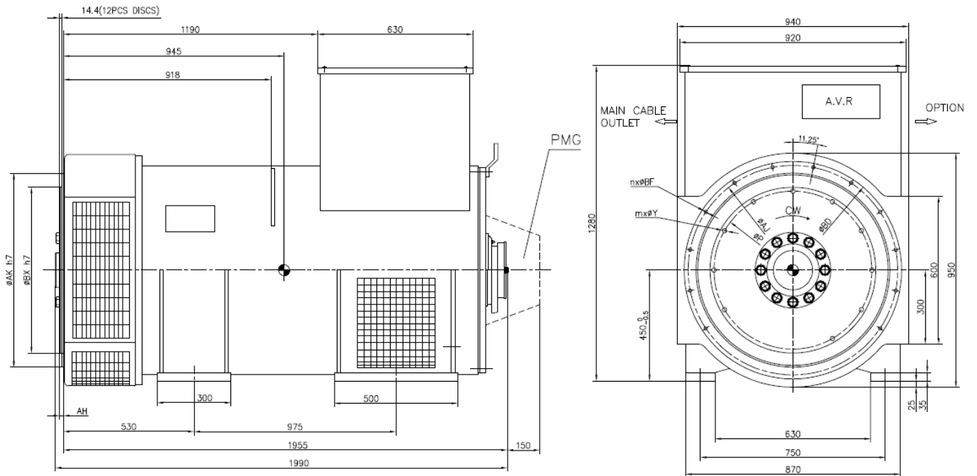
Flange dimensions
