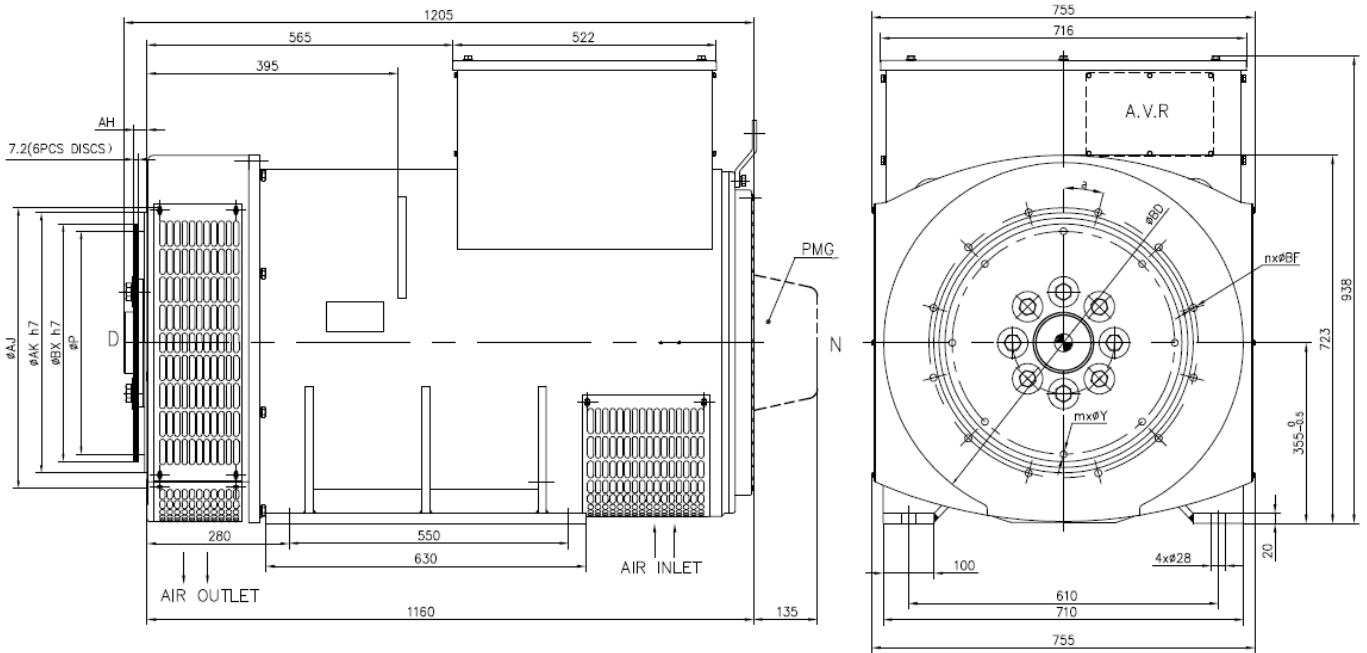
Flange dimensions
