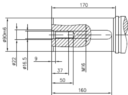
SHAFT END DIMENSIONS
