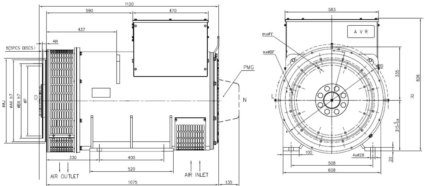
Flange dimensions
