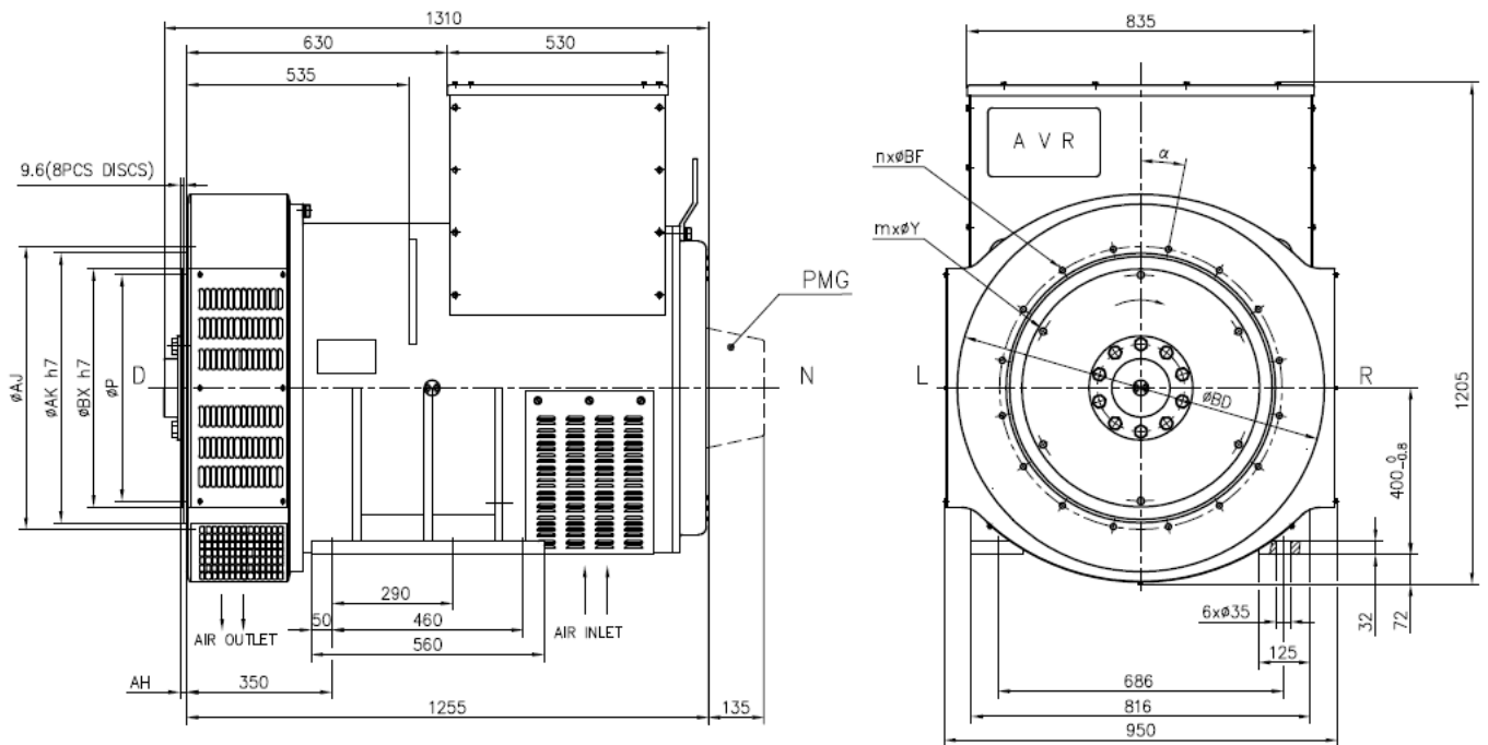
Flange dimensions
