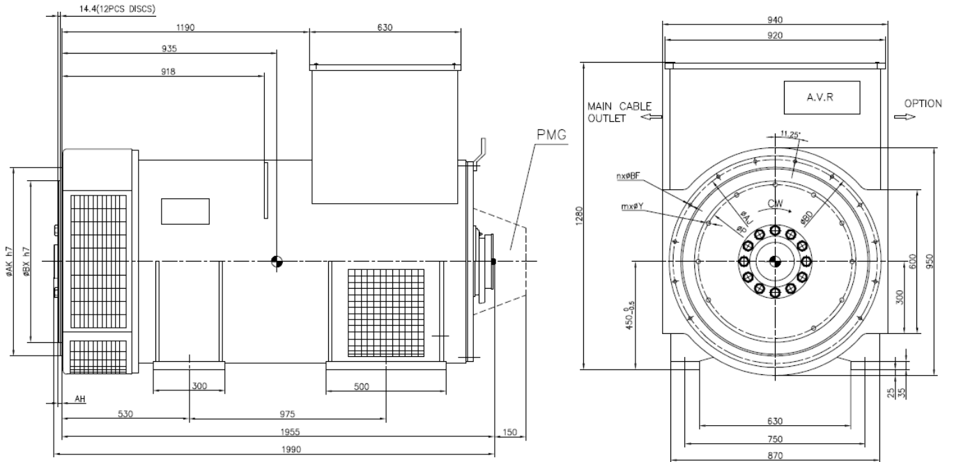
Flange dimensions
