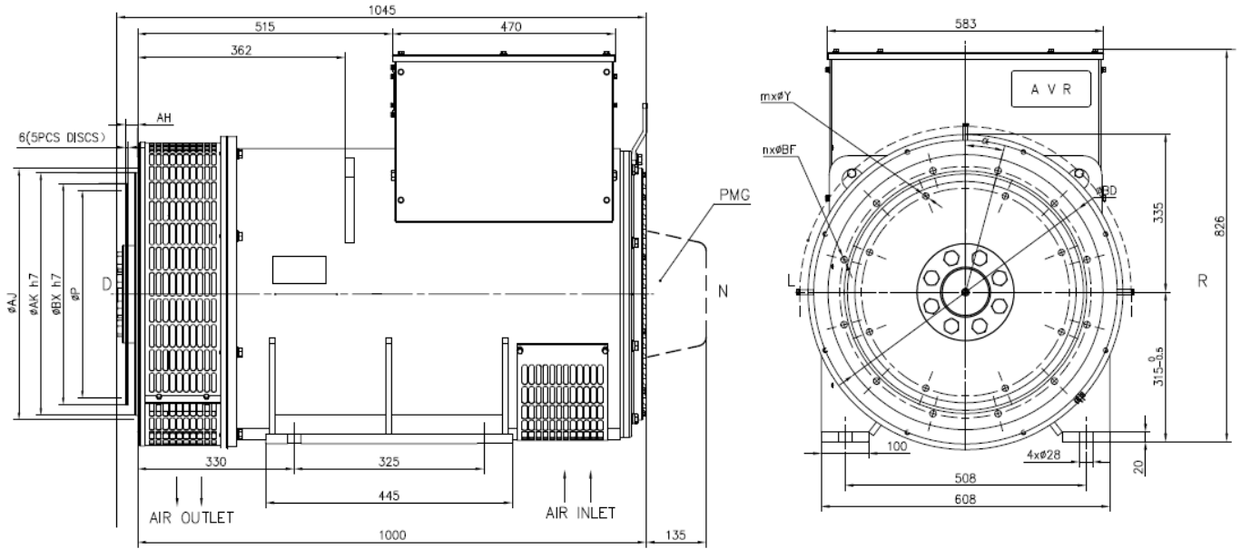
Flange dimensions
