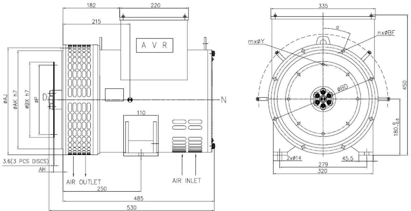
Flange dimensions
