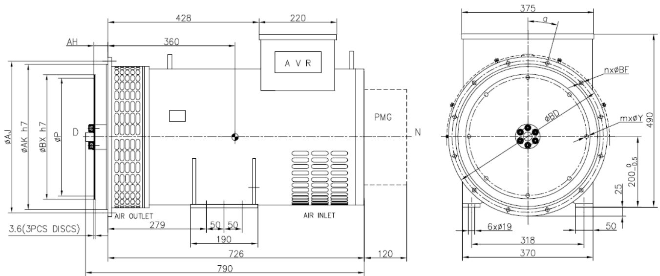
Flange dimensions
