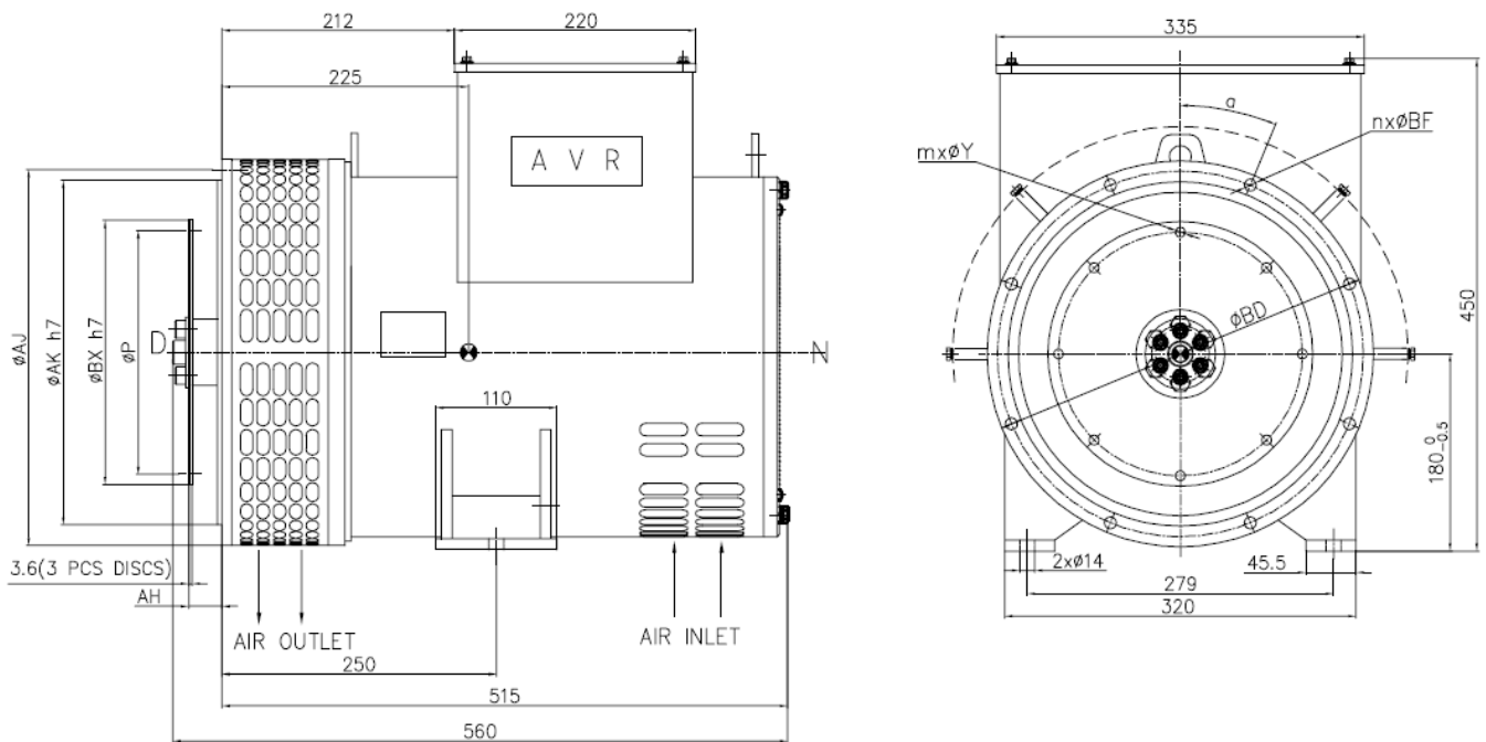
Flange dimensions
