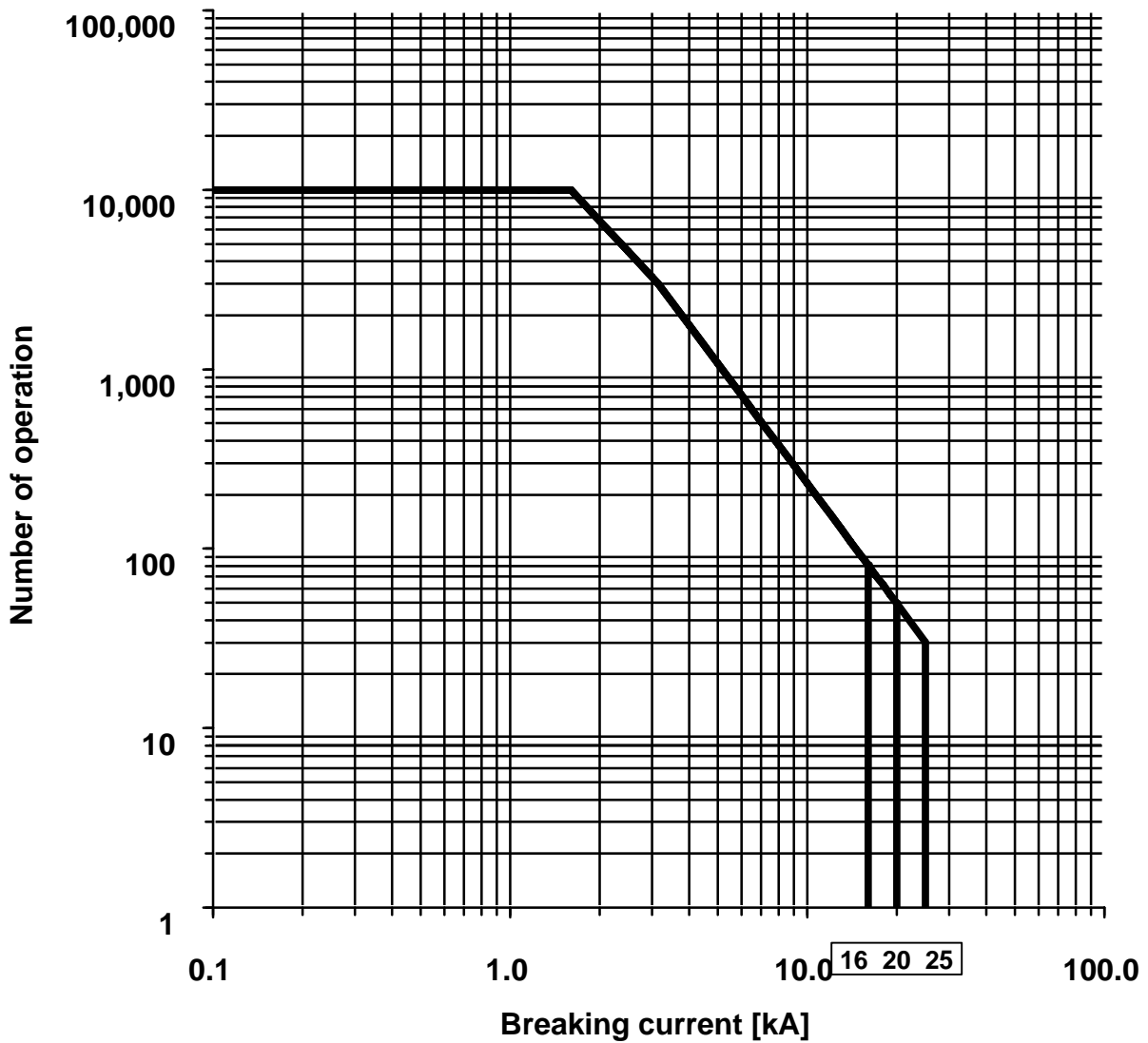
Permissible number of switching operations in relation to breaking current
