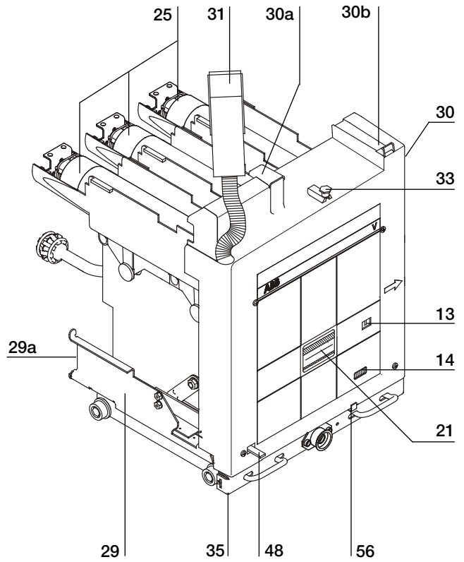
V/ZC contactor for CBE1 enclosures and ZS1 switchboards
