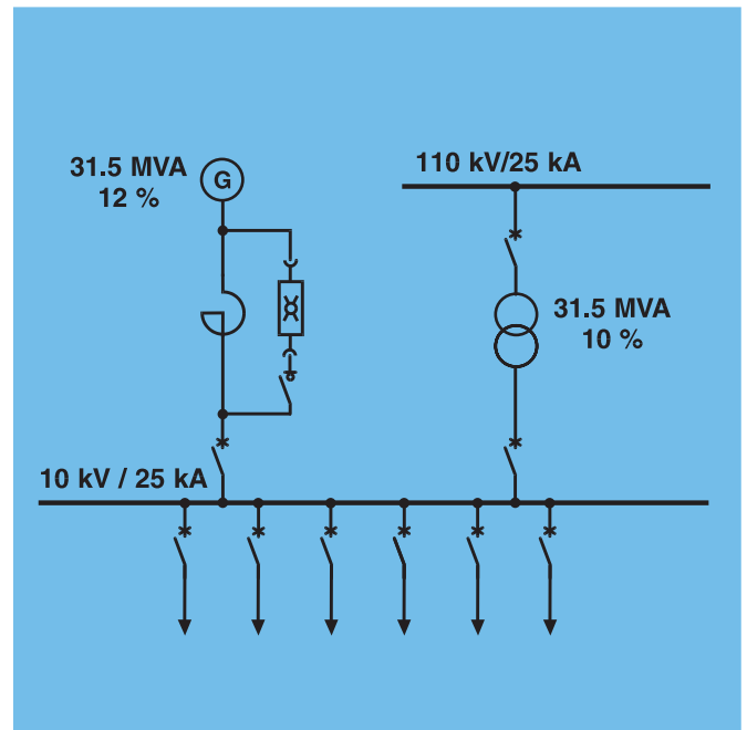
Figure 11: I_s -limiter in parallel with a reactor in a generator feeder
