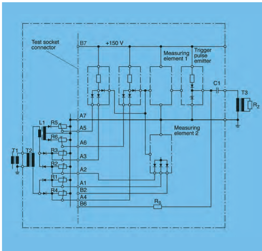
Figure 5: Schematic diagram of a measuring and tripping unit
