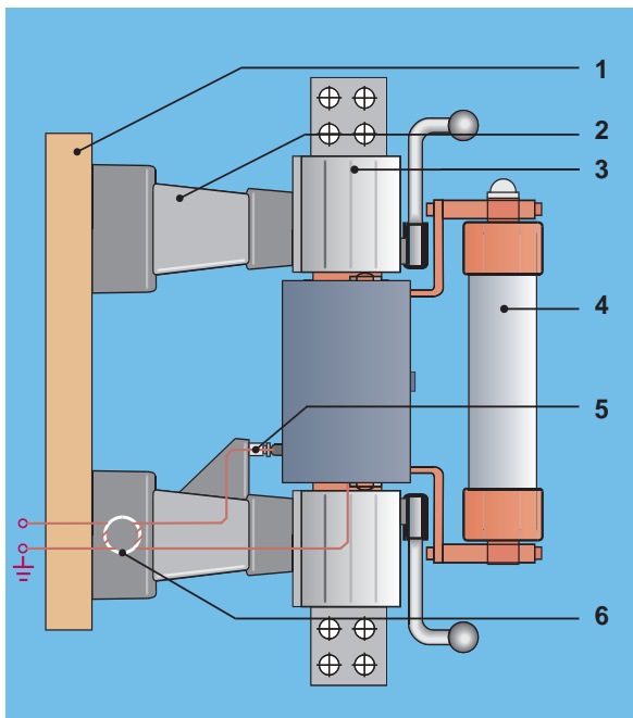
Figure 1: I_s -limiter insert holder with insert for 12 kV, 2000 A
