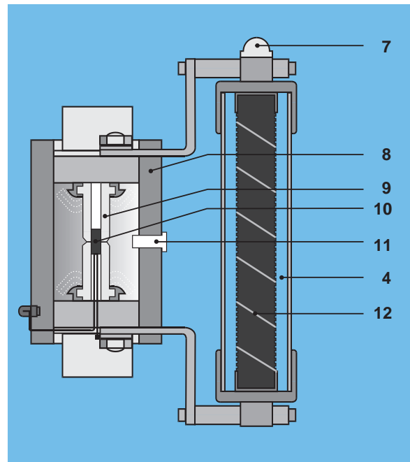
Figure 2: I_s -limiter insert
