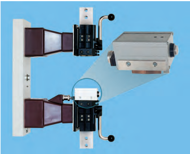
Figure 6: I_s -limiter insert holder with test insert
