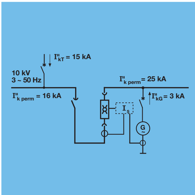
Figure 10: I_s -limiter in connecting point with a public supply network
