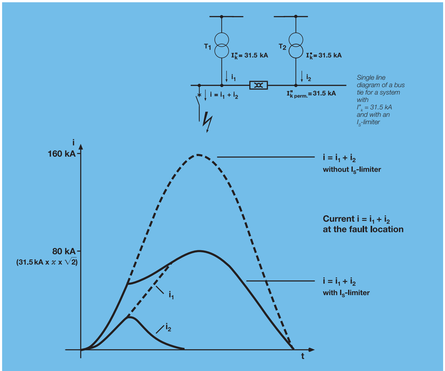
Current i = i_1 + i_2 at the fault location
