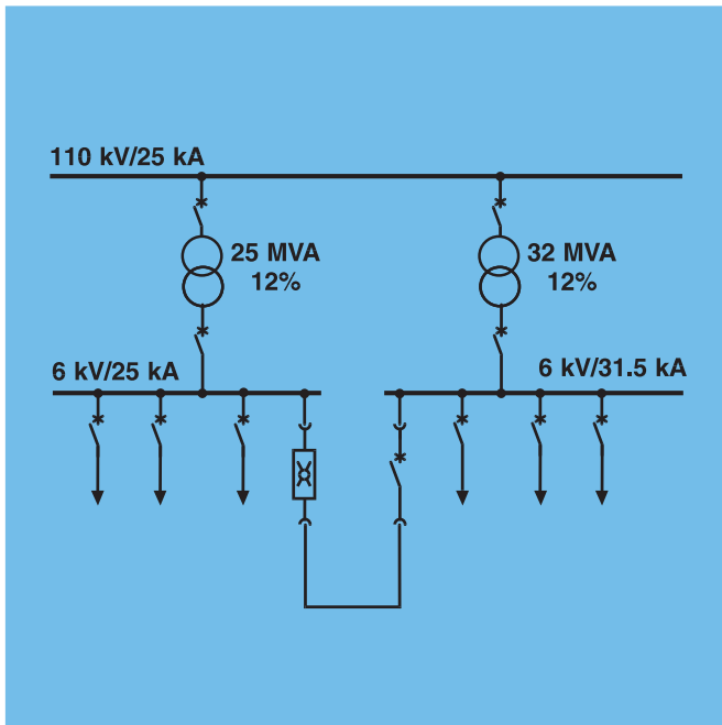
Figure 9: I_s -limiter in a bus section
