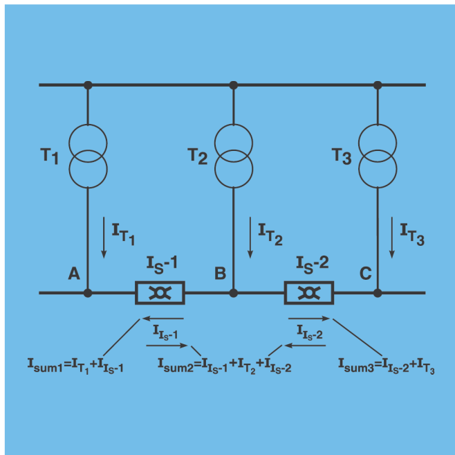
Figure 12: Schematic diagram- I_S -limiter with summation of currents
