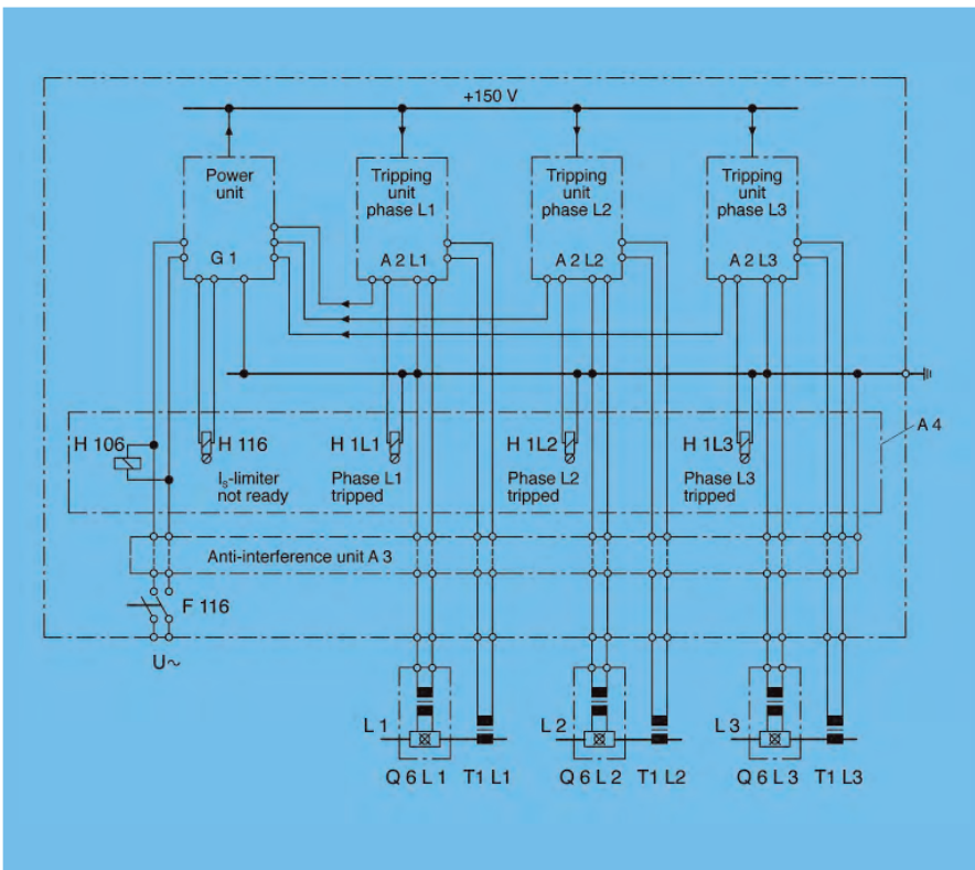
Figure 4: Schematic diagram of the I_s -limiter equipment
