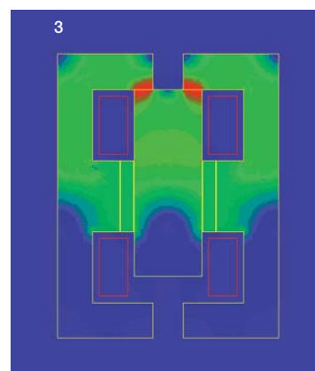
1 Magnetic latching in a limit position. | 2 Magnetic latching plus current build up in one coil. | 3 Armature reaching the opposite limit position.
