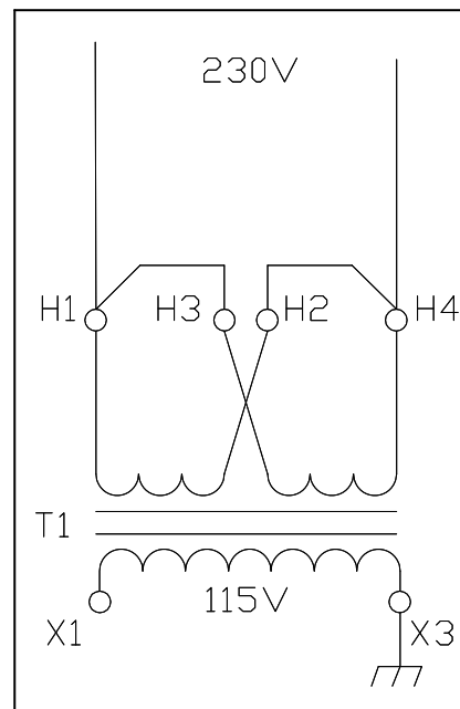
230V reconnection
