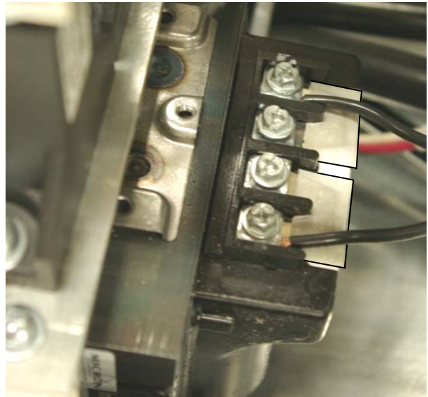
After (230V)
