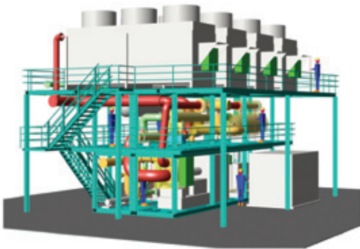
Figure 6. Layout of the ABB ORC power plant.
